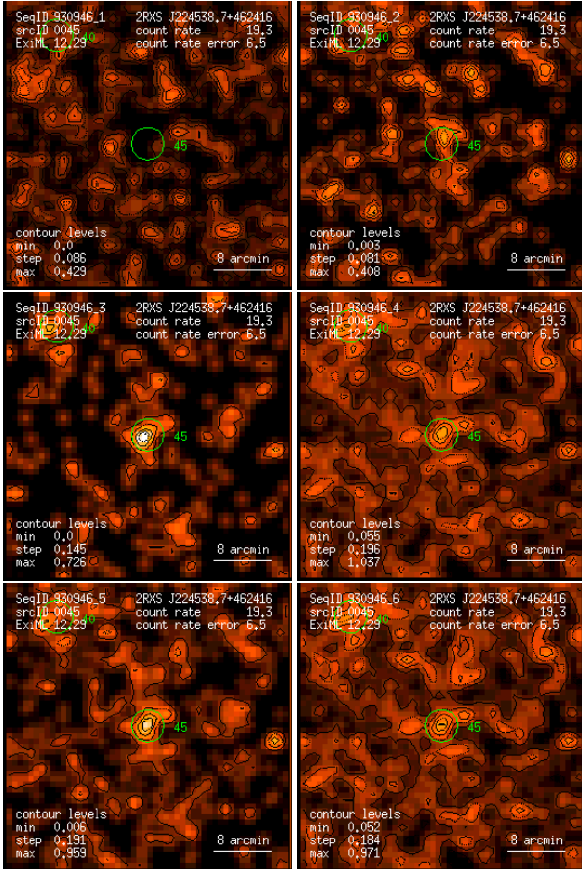
Figure 45: RASS 930946: detection 0045: band rate images, Gaussian filter: (1) PSPC channels 11 – 41, (2) 52 – 90, (3) 91 – 201, (4) 11 – 235, (5) 52 – 201, (6) 11 – 201. Broad band rates in counts/ks. Band rate contour levels in counts/ks/arcmin 2 .
