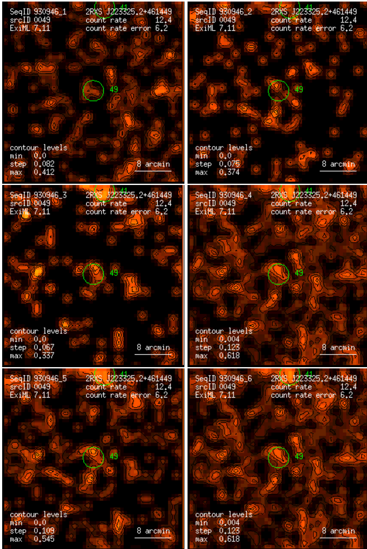
Figure 49: RASS 930946: detection 0049: band rate images, Gaussian filter: (1) PSPC channels 11 – 41, (2) 52 – 90, (3) 91 – 201, (4) 11 – 235, (5) 52 – 201, (6) 11 – 201. Broad band rates in counts/ks. Band rate contour levels in counts/ks/arcmin 2 .
