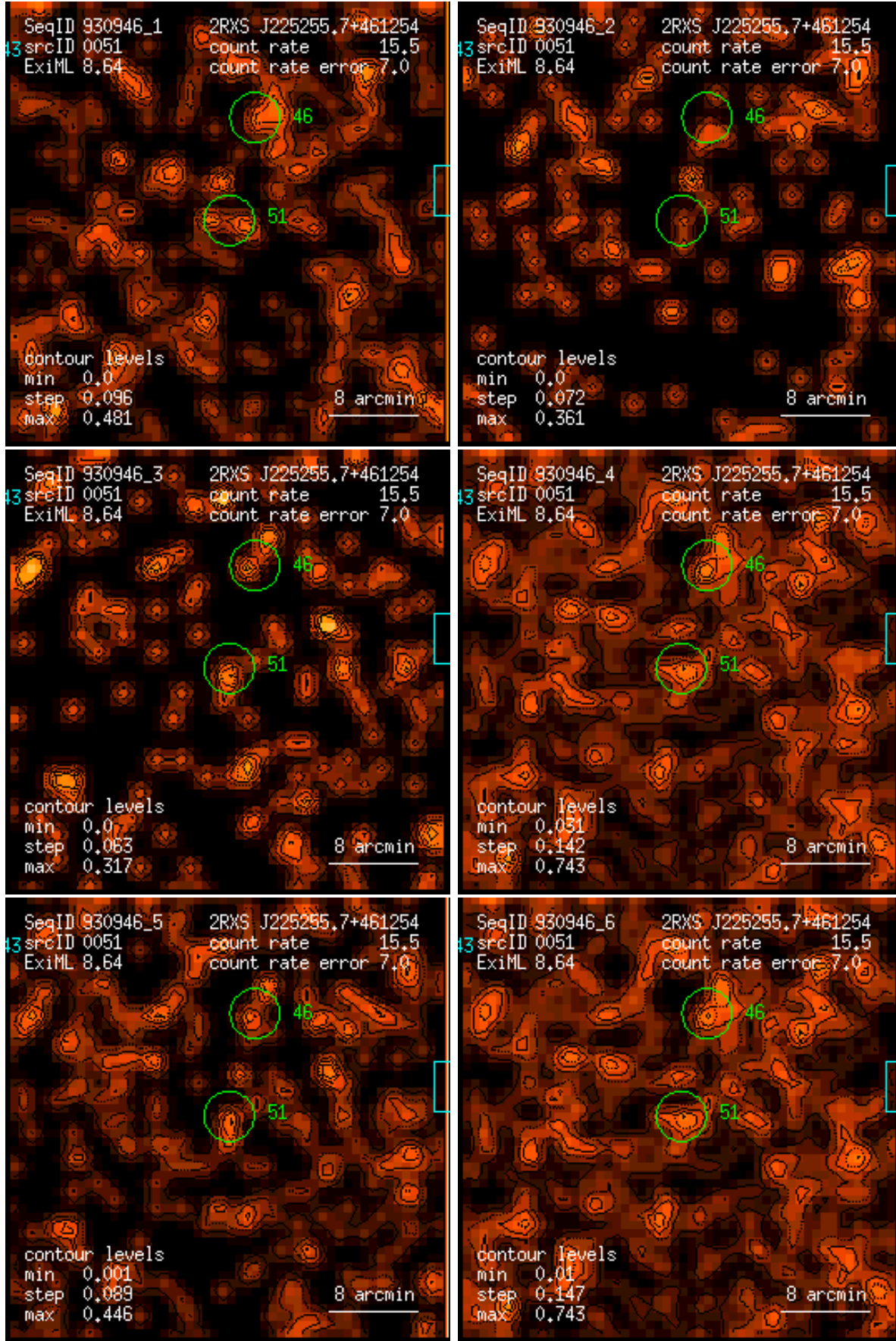
Figure 51: RASS 930946: detection 0051: band rate images, Gaussian filter: (1) PSPC channels 11 – 41, (2) 52 – 90, (3) 91 – 201, (4) 11 – 235, (5) 52 – 201, (6) 11 – 201. Broad band rates in counts/ks. Band rate contour levels in counts/ks/arcmin 2 .
