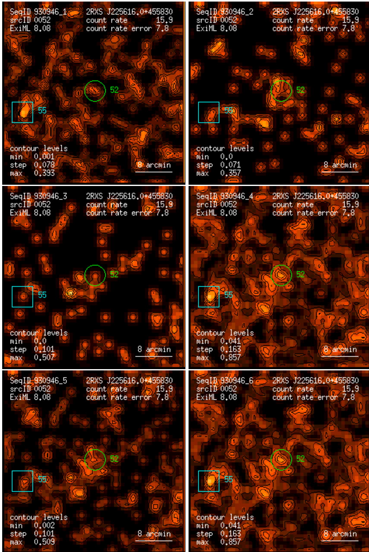
Figure 52: RASS 930946: detection 0052: band rate images, Gaussian filter: (1) PSPC channels 11 – 41, (2) 52 – 90, (3) 91 – 201, (4) 11 – 235, (5) 52 – 201, (6) 11 – 201. Broad band rates in counts/ks. Band rate contour levels in counts/ks/arcmin 2 .
