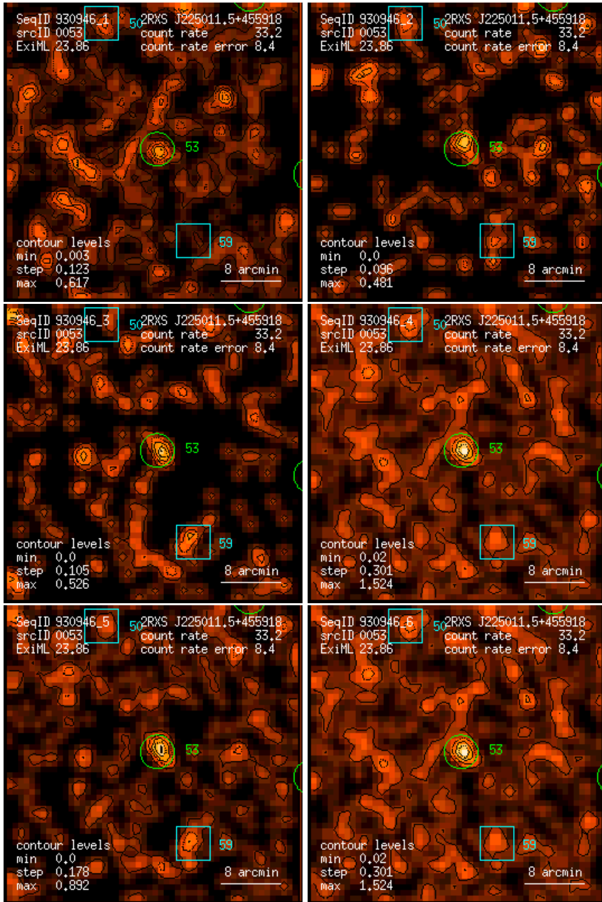
Figure 53: RASS 930946: detection 0053: band rate images, Gaussian filter: (1) PSPC channels 11 – 41, (2) 52 – 90, (3) 91 – 201, (4) 11 – 235, (5) 52 – 201, (6) 11 – 201. Broad band rates in counts/ks. Band rate contour levels in counts/ks/arcmin 2 .
