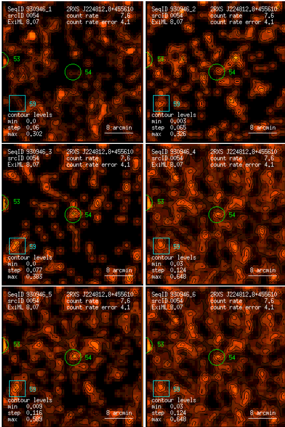
Figure 54: RASS 930946: detection 0054: band rate images, Gaussian filter: (1) PSPC channels 11 – 41, (2) 52 – 90, (3) 91 – 201, (4) 11 – 235, (5) 52 – 201, (6) 11 – 201. Broad band rates in counts/ks. Band rate contour levels in counts/ks/arcmin 2 .
