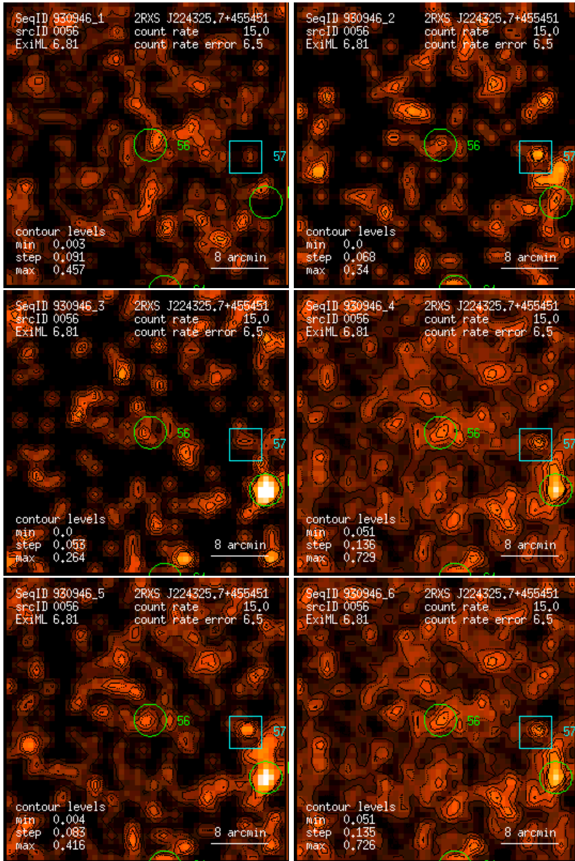
Figure 56: RASS 930946: detection 0056: band rate images, Gaussian filter: (1) PSPC channels 11 – 41, (2) 52 – 90, (3) 91 – 201, (4) 11 – 235, (5) 52 – 201, (6) 11 – 201. Broad band rates in counts/ks. Band rate contour levels in counts/ks/arcmin 2 .
