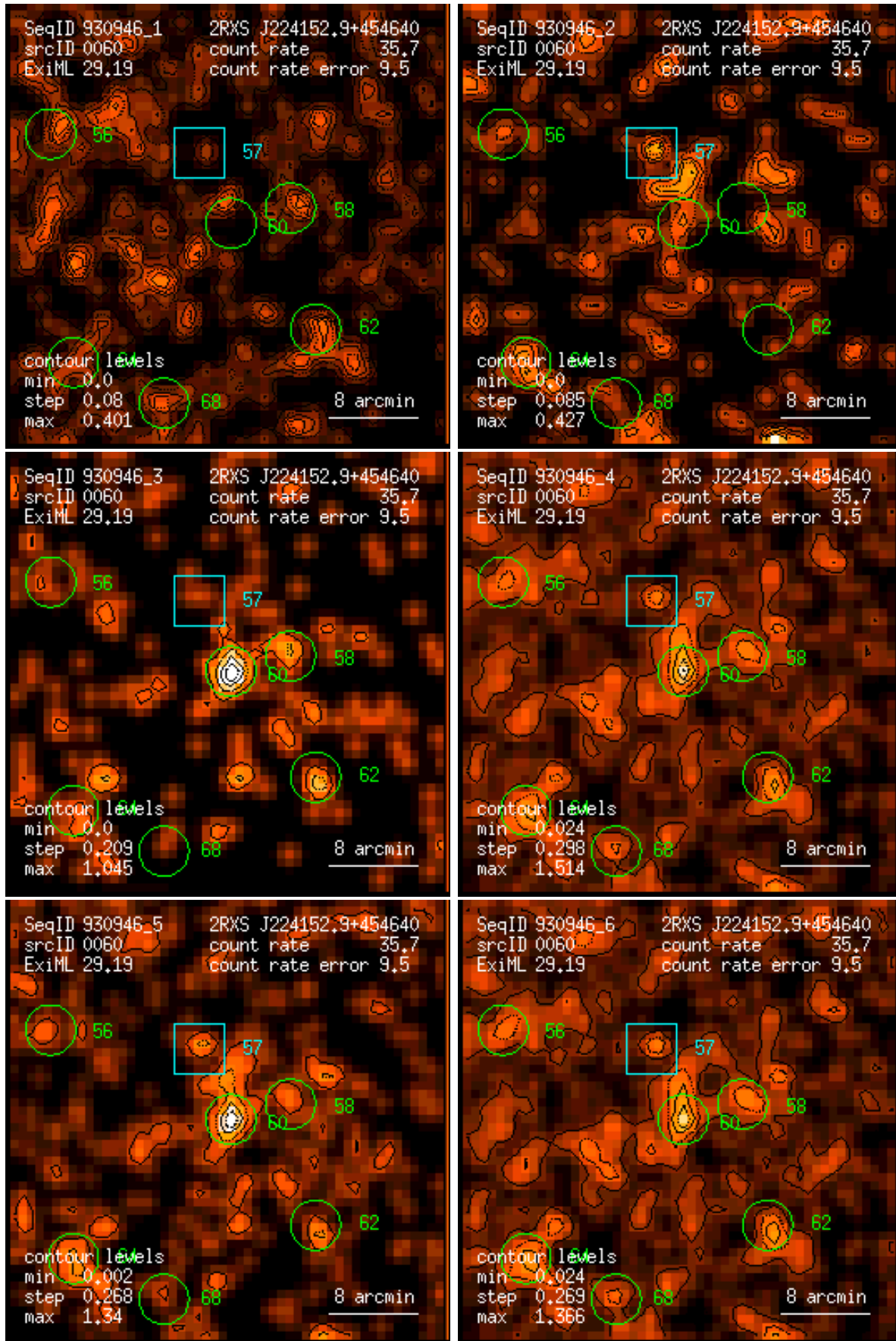
Figure 60: RASS 930946: detection 0060: band rate images, Gaussian filter: (1) PSPC channels 11 – 41, (2) 52 – 90, (3) 91 – 201, (4) 11 – 235, (5) 52 – 201, (6) 11 – 201. Broad band rates in counts/ks. Band rate contour levels in counts/ks/arcmin 2 .
