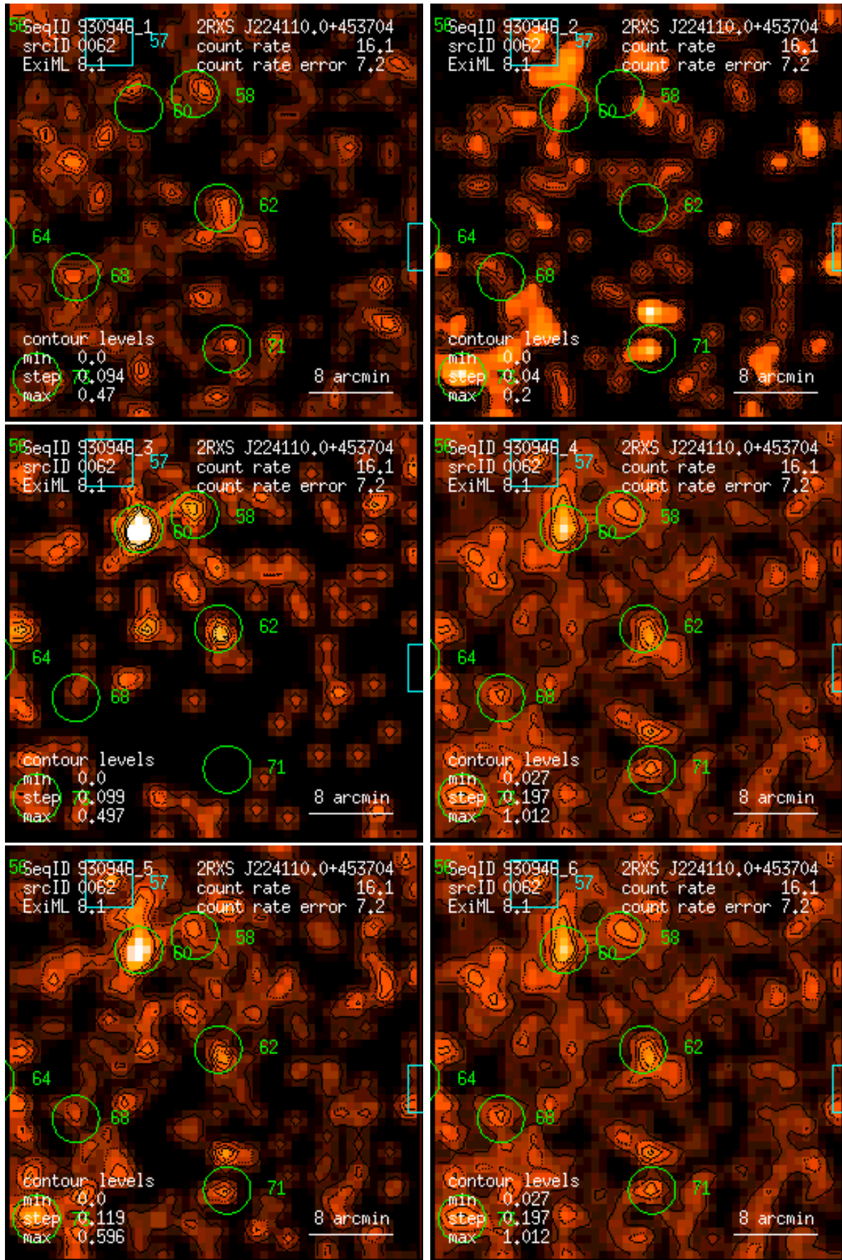
Figure 62: RASS 930946: detection 0062: band rate images, Gaussian filter: (1) PSPC channels 11 – 41, (2) 52 – 90, (3) 91 – 201, (4) 11 – 235, (5) 52 – 201, (6) 11 – 201. Broad band rates in counts/ks. Band rate contour levels in counts/ks/arcmin 2 .
