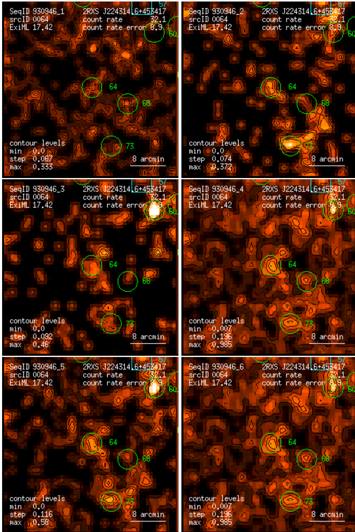
Figure 64: RASS 930946: detection 0064: band rate images, Gaussian filter: (1) PSPC channels 11 – 41, (2) 52 – 90, (3) 91 – 201, (4) 11 – 235, (5) 52 – 201, (6) 11 – 201. Broad band rates in counts/ks. Band rate contour levels in counts/ks/arcmin 2 .
