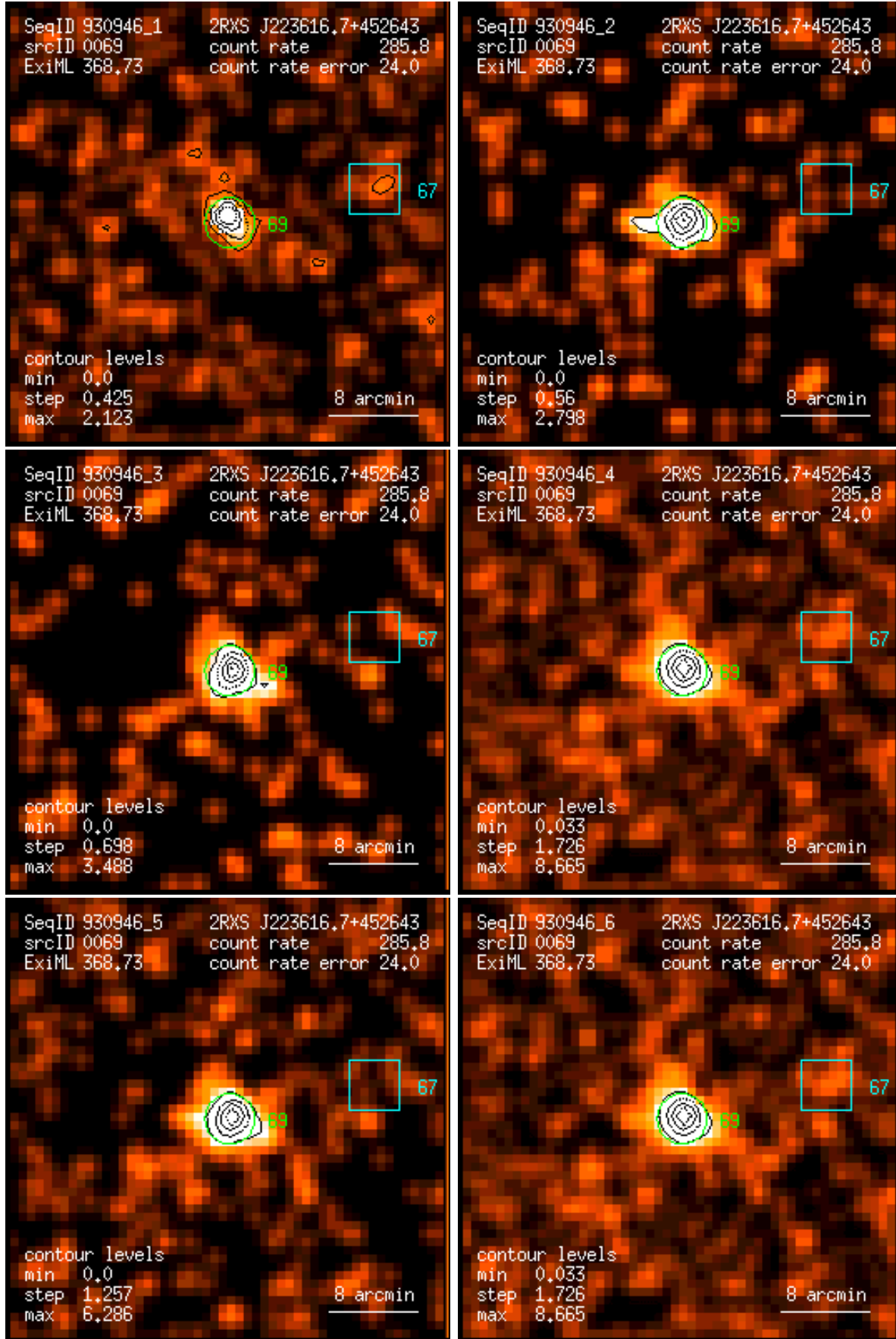
Figure 69: RASS 930946: detection 0069: band rate images, Gaussian filter: (1) PSPC channels 11 – 41, (2) 52 – 90, (3) 91 – 201, (4) 11 – 235, (5) 52 – 201, (6) 11 – 201. Broad band rates in counts/ks. Band rate contour levels in counts/ks/arcmin 2 .
