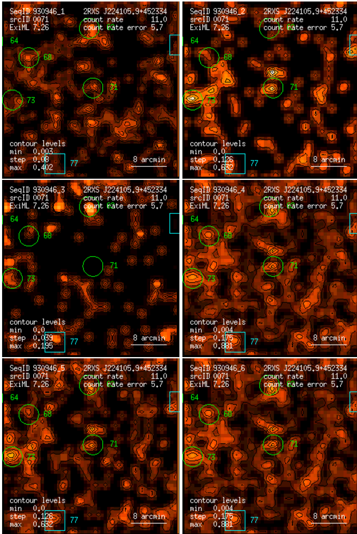
Figure 71: RASS 930946: detection 0071: band rate images, Gaussian filter: (1) PSPC channels 11 – 41, (2) 52 – 90, (3) 91 – 201, (4) 11 – 235, (5) 52 – 201, (6) 11 – 201. Broad band rates in counts/ks. Band rate contour levels in counts/ks/arcmin 2 .
