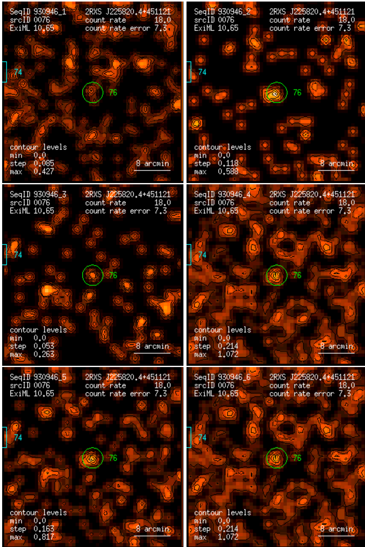
Figure 76: RASS 930946: detection 0076: band rate images, Gaussian filter: (1) PSPC channels 11 – 41, (2) 52 – 90, (3) 91 – 201, (4) 11 – 235, (5) 52 – 201, (6) 11 – 201. Broad band rates in counts/ks. Band rate contour levels in counts/ks/arcmin 2 .
