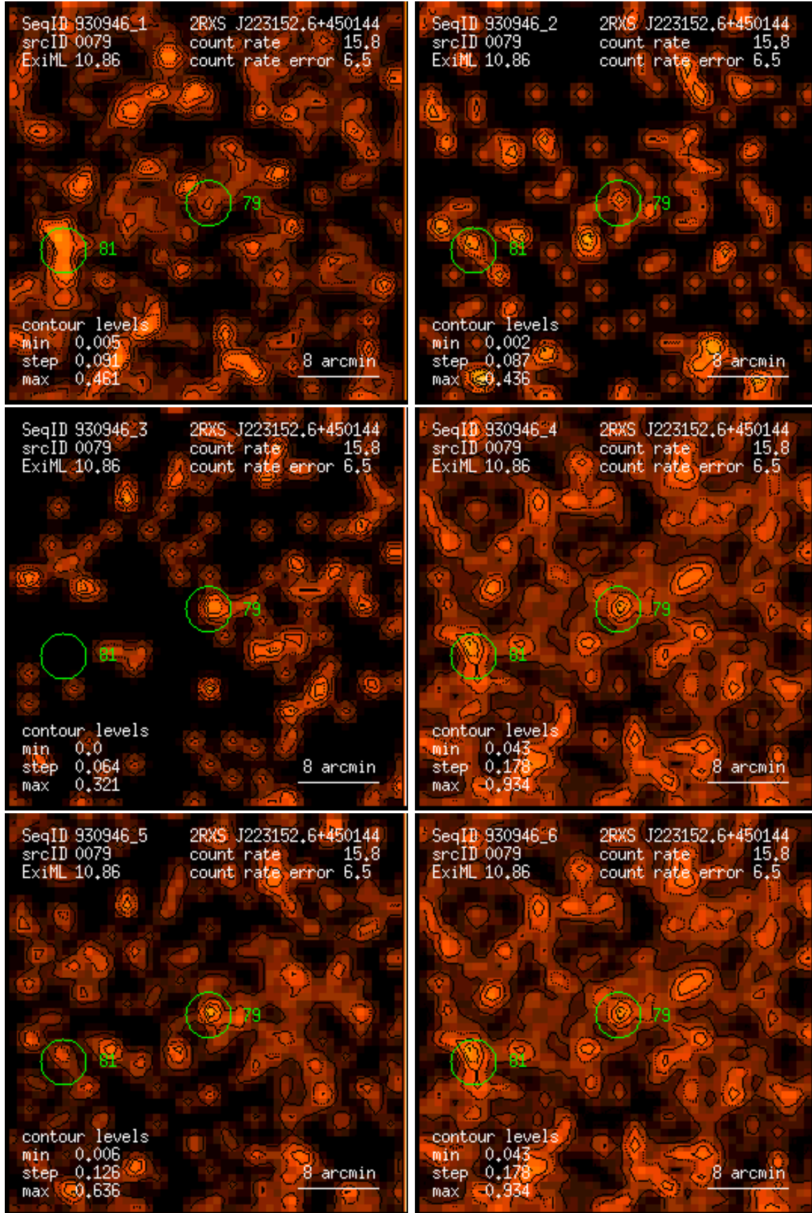
Figure 79: RASS 930946: detection 0079: band rate images, Gaussian filter: (1) PSPC channels 11 – 41, (2) 52 – 90, (3) 91 – 201, (4) 11 – 235, (5) 52 – 201, (6) 11 – 201. Broad band rates in counts/ks. Band rate contour levels in counts/ks/arcmin 2 .
