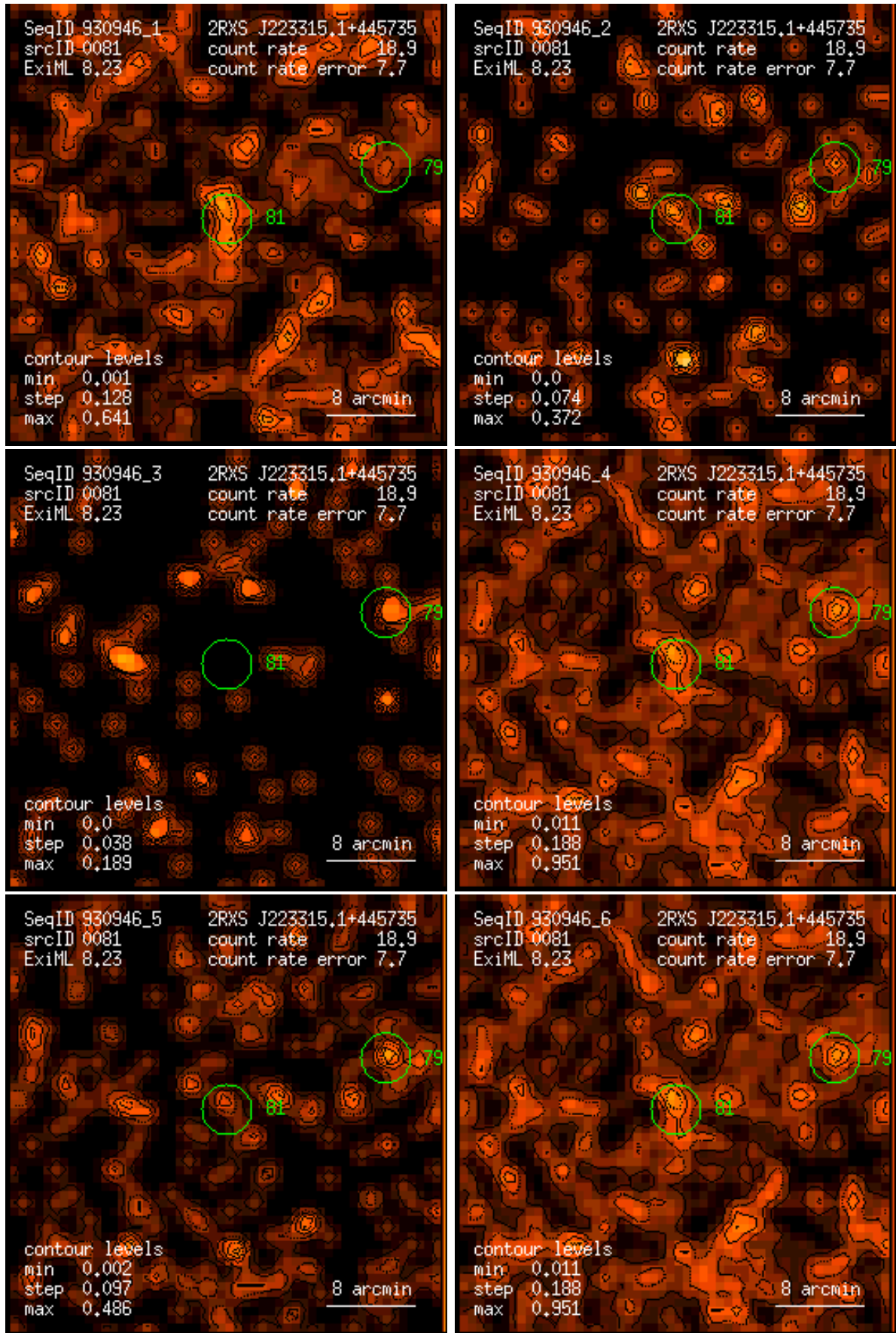
Figure 81: RASS 930946: detection 0081: band rate images, Gaussian filter: (1) PSPC channels 11 – 41, (2) 52 – 90, (3) 91 – 201, (4) 11 – 235, (5) 52 – 201, (6) 11 – 201. Broad band rates in counts/ks. Band rate contour levels in counts/ks/arcmin 2 .
