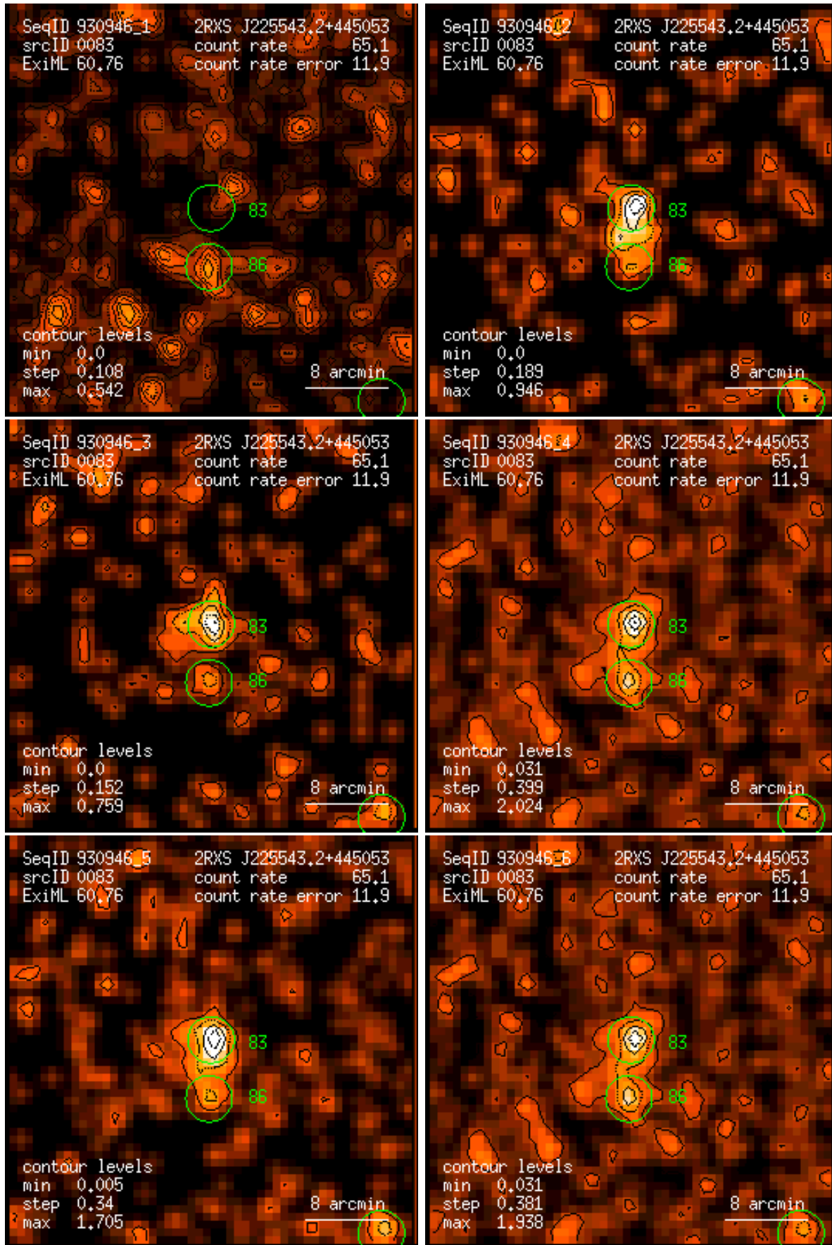
Figure 83: RASS 930946: detection 0083: band rate images, Gaussian filter: (1) PSPC channels 11 – 41, (2) 52 – 90, (3) 91 – 201, (4) 11 – 235, (5) 52 – 201, (6) 11 – 201. Broad band rates in counts/ks. Band rate contour levels in counts/ks/arcmin 2 .
