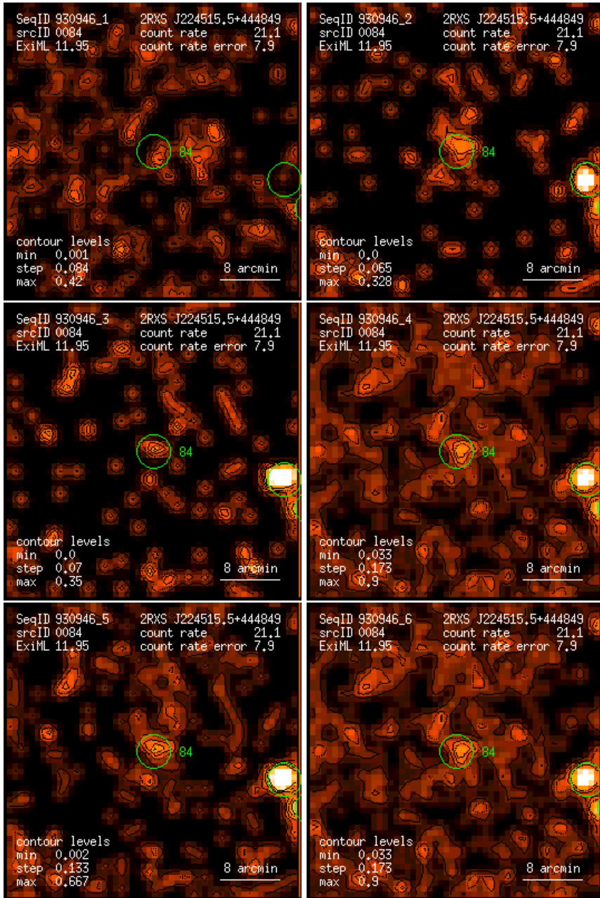
Figure 84: RASS 930946: detection 0084: band rate images, Gaussian filter: (1) PSPC channels 11 – 41, (2) 52 – 90, (3) 91 – 201, (4) 11 – 235, (5) 52 – 201, (6) 11 – 201. Broad band rates in counts/ks. Band rate contour levels in counts/ks/arcmin 2 .
