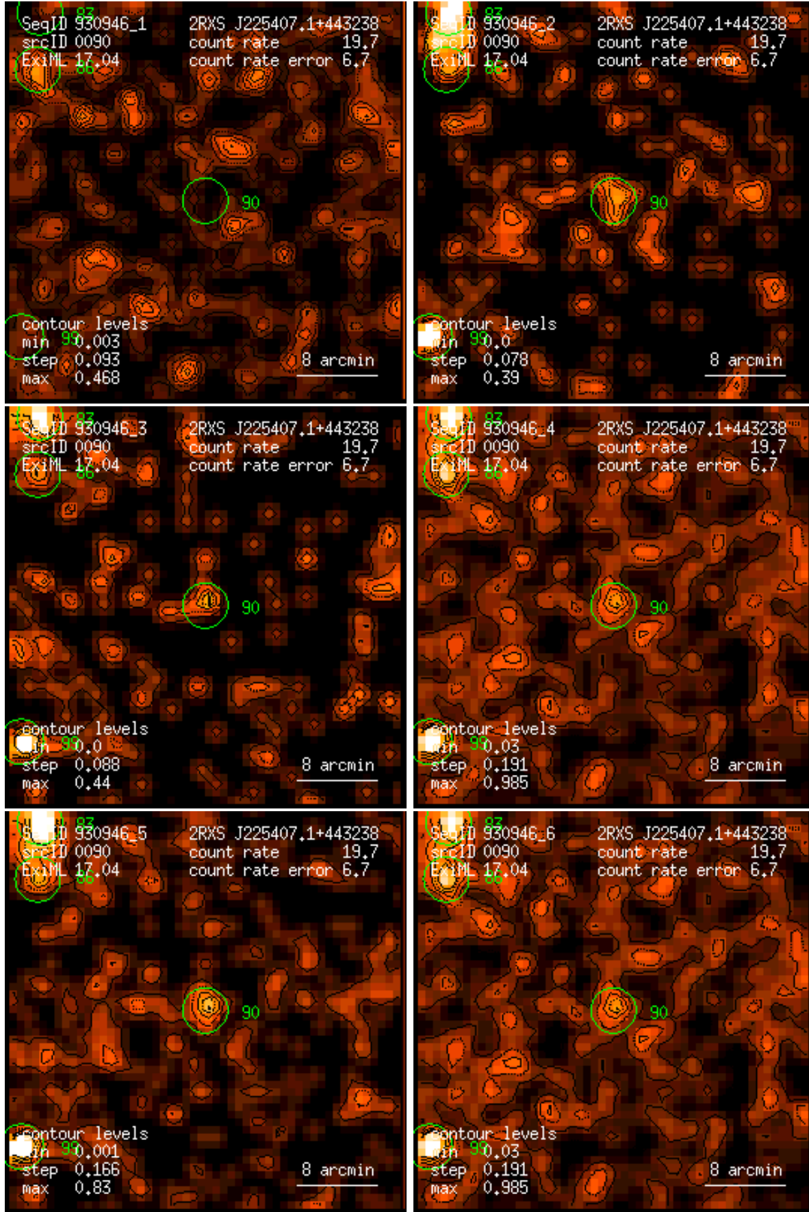
Figure 90: RASS 930946: detection 0090: band rate images, Gaussian filter: (1) PSPC channels 11 – 41, (2) 52 – 90, (3) 91 – 201, (4) 11 – 235, (5) 52 – 201, (6) 11 – 201. Broad band rates in counts/ks. Band rate contour levels in counts/ks/arcmin 2 .
