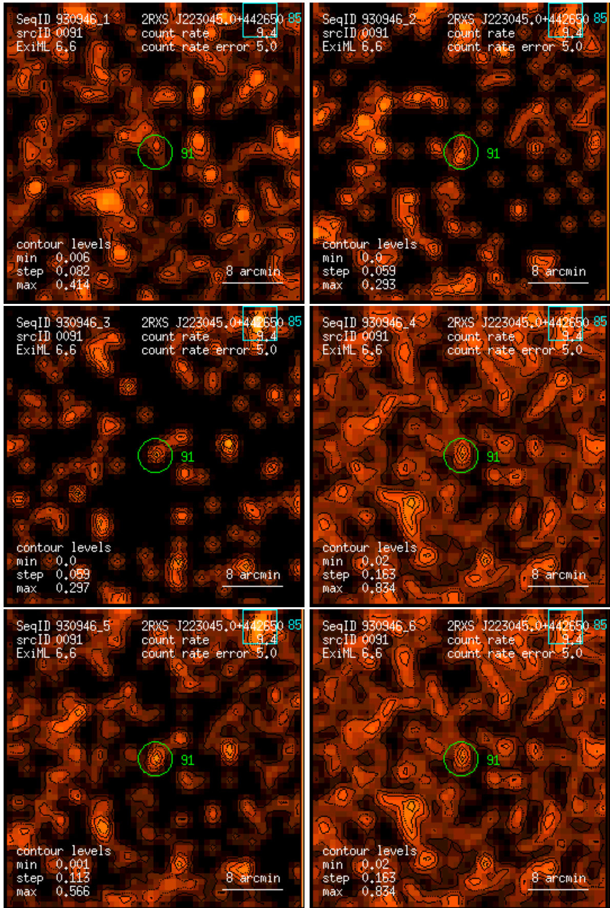
Figure 91: RASS 930946: detection 0091: band rate images, Gaussian filter: (1) PSPC channels 11 – 41, (2) 52 – 90, (3) 91 – 201, (4) 11 – 235, (5) 52 – 201, (6) 11 – 201. Broad band rates in counts/ks. Band rate contour levels in counts/ks/arcmin 2 .
