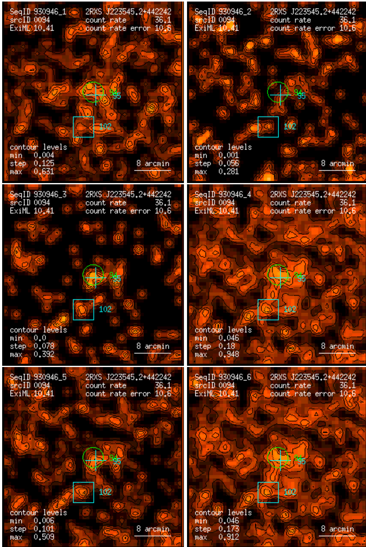
Figure 94: RASS 930946: detection 0094: band rate images, Gaussian filter: (1) PSPC channels 11 – 41, (2) 52 – 90, (3) 91 – 201, (4) 11 – 235, (5) 52 – 201, (6) 11 – 201. Broad band rates in counts/ks. Band rate contour levels in counts/ks/arcmin 2 .
