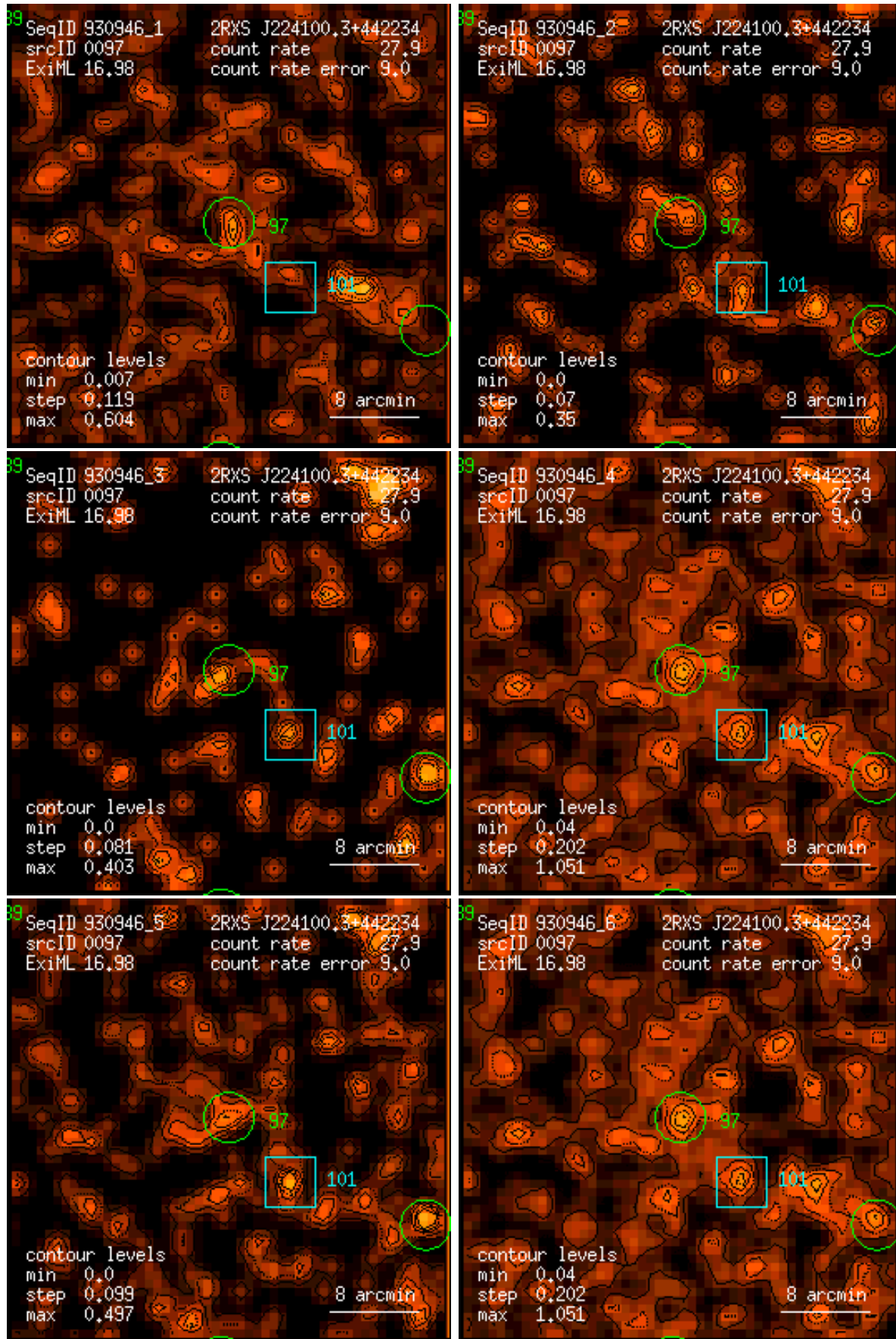
Figure 97: RASS 930946: detection 0097: band rate images, Gaussian filter: (1) PSPC channels 11 – 41, (2) 52 – 90, (3) 91 – 201, (4) 11 – 235, (5) 52 – 201, (6) 11 – 201. Broad band rates in counts/ks. Band rate contour levels in counts/ks/arcmin 2 .
