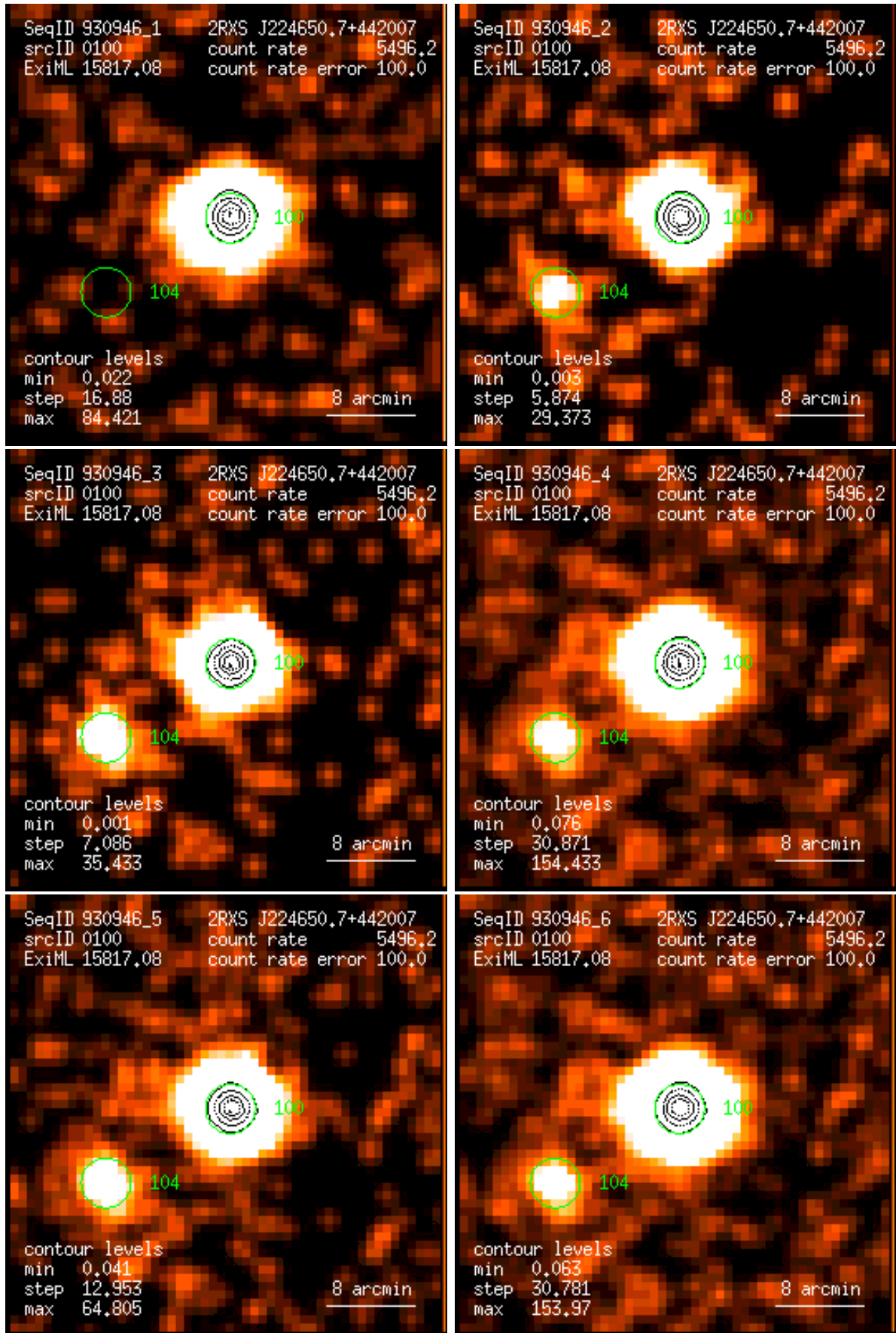
Figure 100: RASS 930946: detection 0100: band rate images, Gaussian filter: (1) PSPC channels 11 – 41, (2) 52 – 90, (3) 91 – 201, (4) 11 – 235, (5) 52 – 201, (6) 11 – 201. Broad band rates in counts/ks. Band rate contour levels in counts/ks/arcmin 2 .
