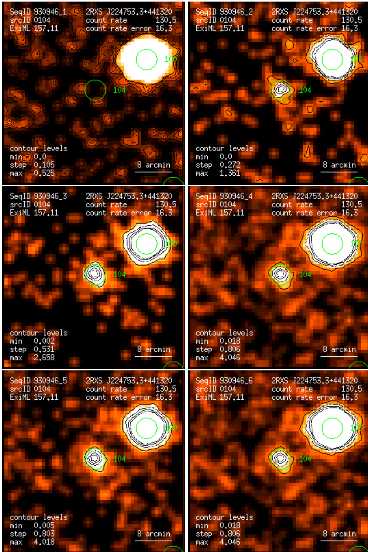
Figure 104: RASS 930946: detection 0104: band rate images, Gaussian filter: (1) PSPC channels 11 – 41, (2) 52 – 90, (3) 91 – 201, (4) 11 – 235, (5) 52 – 201, (6) 11 – 201. Broad band rates in counts/ks. Band rate contour levels in counts/ks/arcmin 2 .
