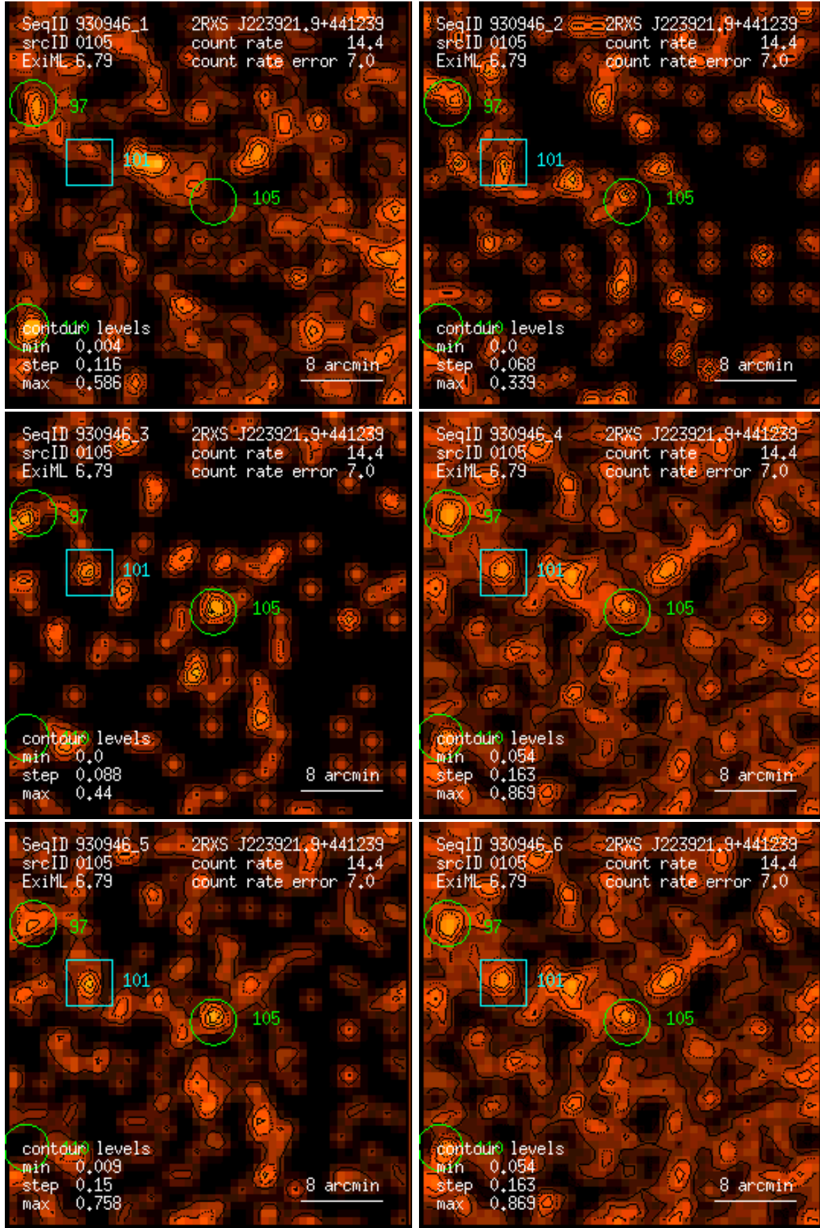
Figure 105: RASS 930946: detection 0105: band rate images, Gaussian filter: (1) PSPC channels 11 – 41, (2) 52 – 90, (3) 91 – 201, (4) 11 – 235, (5) 52 – 201, (6) 11 – 201. Broad band rates in counts/ks. Band rate contour levels in counts/ks/arcmin 2 .
