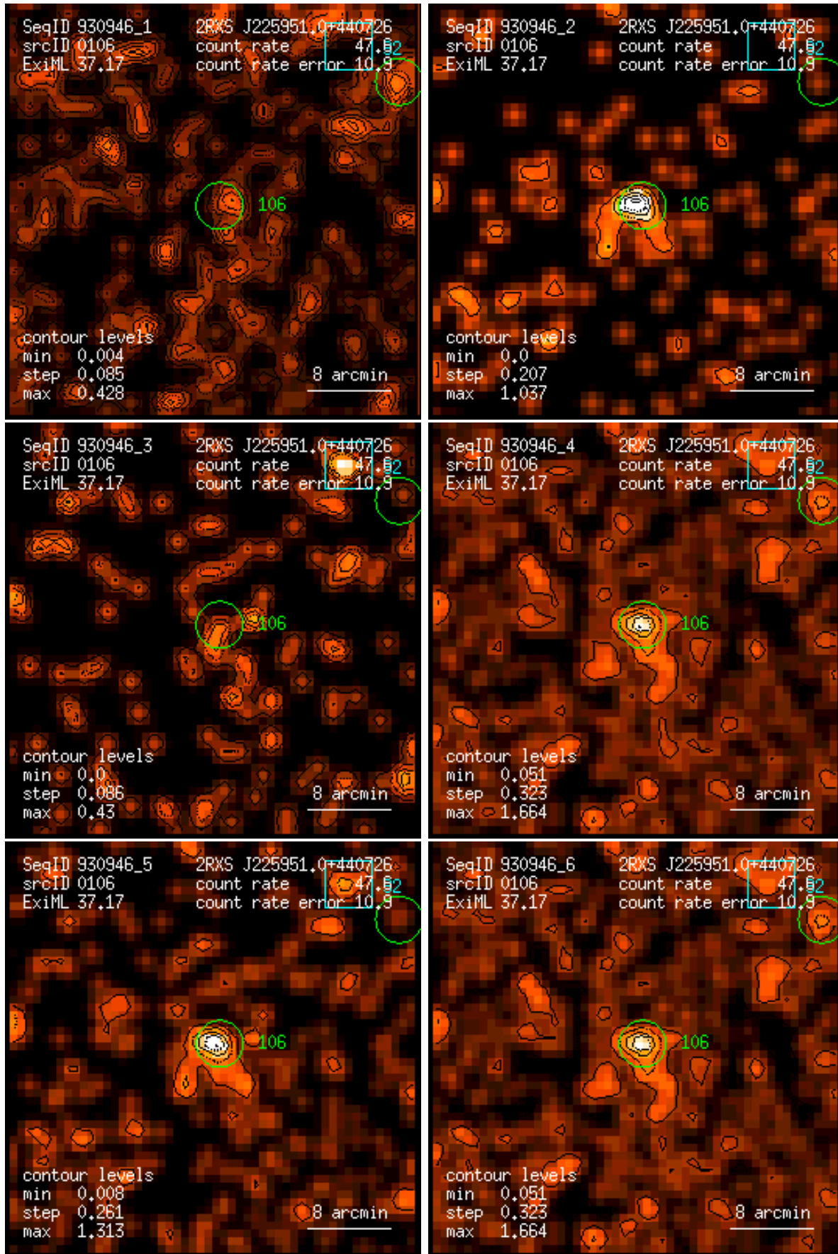
Figure 106: RASS 930946: detection 0106: band rate images, Gaussian filter: (1) PSPC channels 11 – 41, (2) 52 – 90, (3) 91 – 201, (4) 11 – 235, (5) 52 – 201, (6) 11 – 201. Broad band rates in counts/ks. Band rate contour levels in counts/ks/arcmin 2 .
