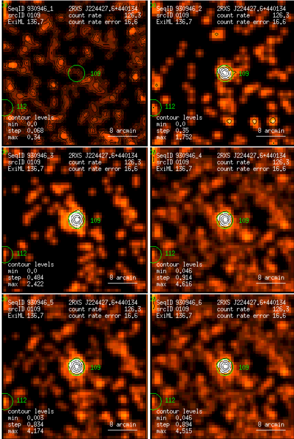
Figure 109: RASS 930946: detection 0109: band rate images, Gaussian filter: (1) PSPC channels 11 – 41, (2) 52 – 90, (3) 91 – 201, (4) 11 – 235, (5) 52 – 201, (6) 11 – 201. Broad band rates in counts/ks. Band rate contour levels in counts/ks/arcmin 2 .
