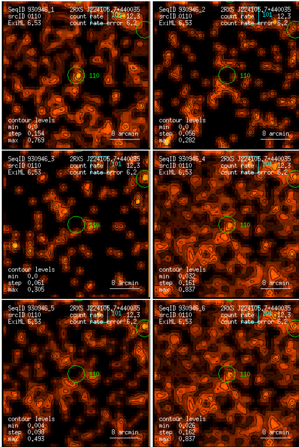
Figure 110: RASS 930946: detection 0110: band rate images, Gaussian filter: (1) PSPC channels 11 – 41, (2) 52 – 90, (3) 91 – 201, (4) 11 – 235, (5) 52 – 201, (6) 11 – 201. Broad band rates in counts/ks. Band rate contour levels in counts/ks/arcmin 2 .
