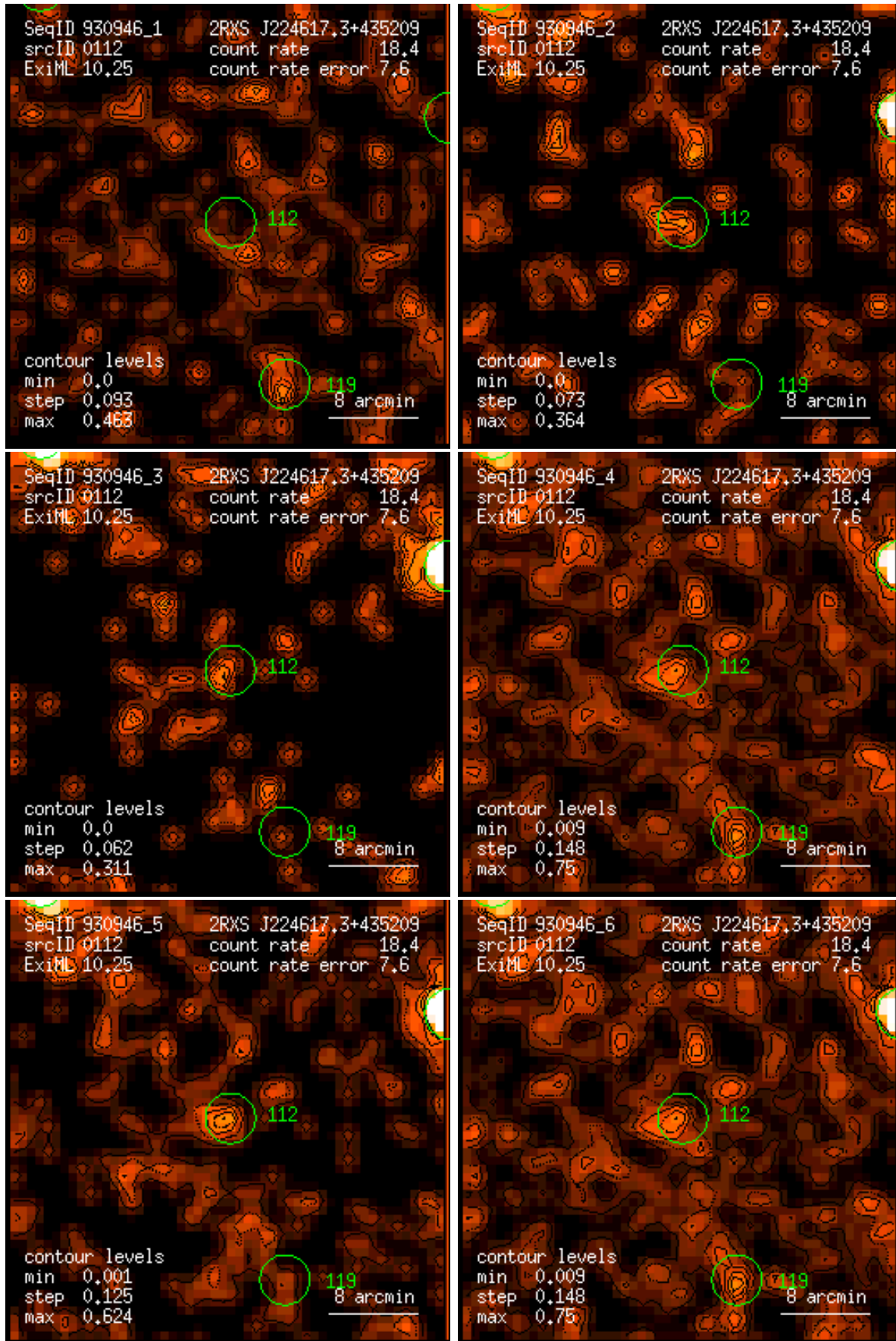
Figure 112: RASS 930946: detection 0112: band rate images, Gaussian filter: (1) PSPC channels 11 – 41, (2) 52 – 90, (3) 91 – 201, (4) 11 – 235, (5) 52 – 201, (6) 11 – 201. Broad band rates in counts/ks. Band rate contour levels in counts/ks/arcmin 2 .
