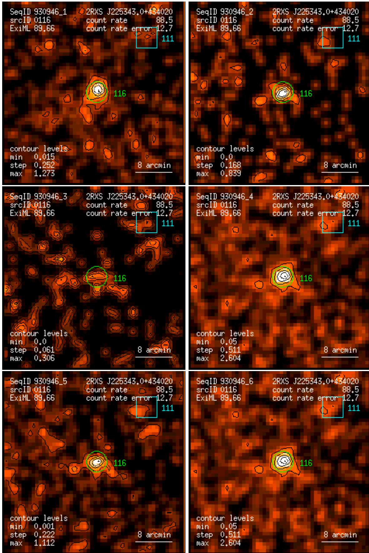
Figure 116: RASS 930946: detection 0116: band rate images, Gaussian filter: (1) PSPC channels 11 – 41, (2) 52 – 90, (3) 91 – 201, (4) 11 – 235, (5) 52 – 201, (6) 11 – 201. Broad band rates in counts/ks. Band rate contour levels in counts/ks/arcmin 2 .
