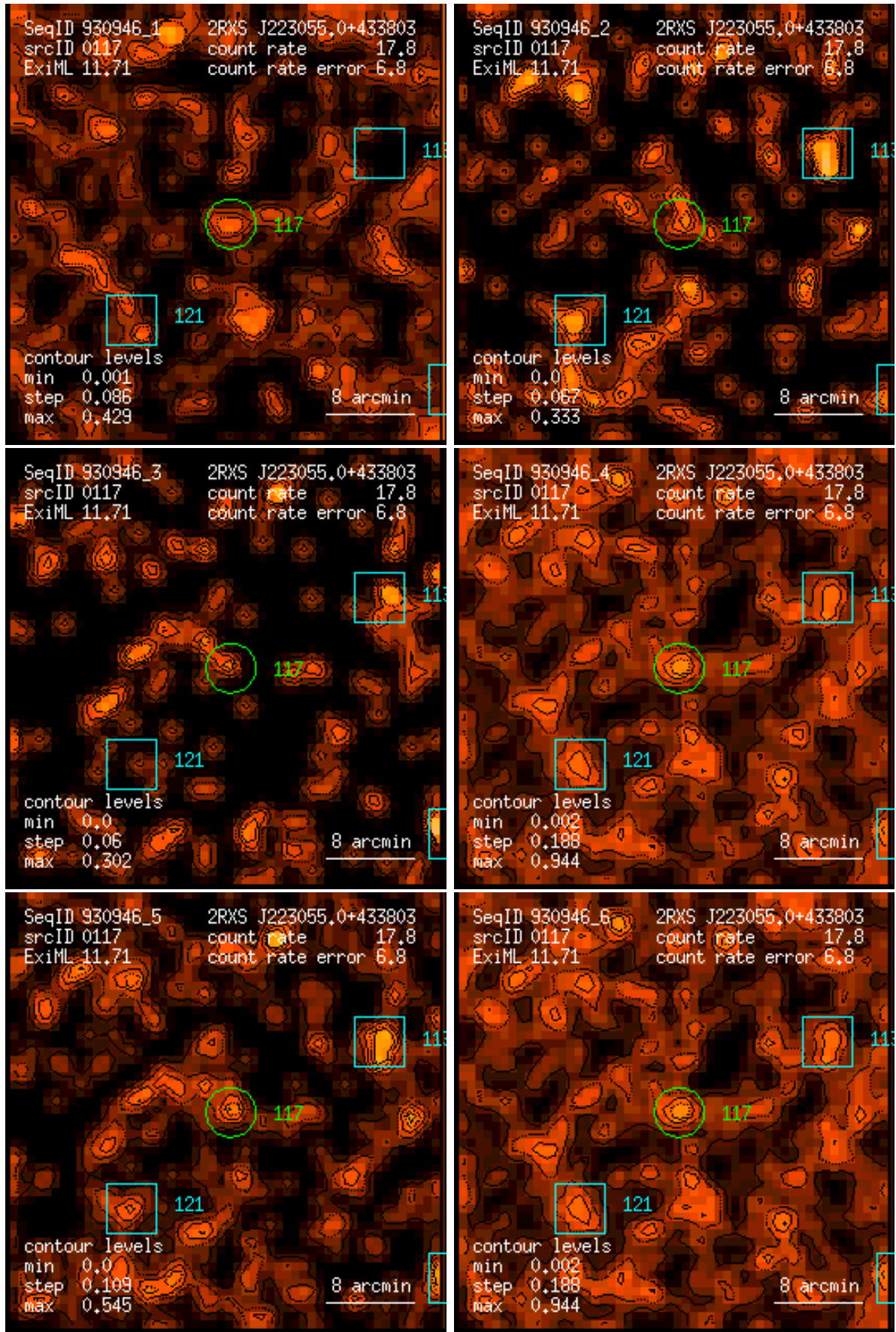
Figure 117: RASS 930946: detection 0117: band rate images, Gaussian filter: (1) PSPC channels 11 – 41, (2) 52 – 90, (3) 91 – 201, (4) 11 – 235, (5) 52 – 201, (6) 11 – 201. Broad band rates in counts/ks. Band rate contour levels in counts/ks/arcmin 2 .
