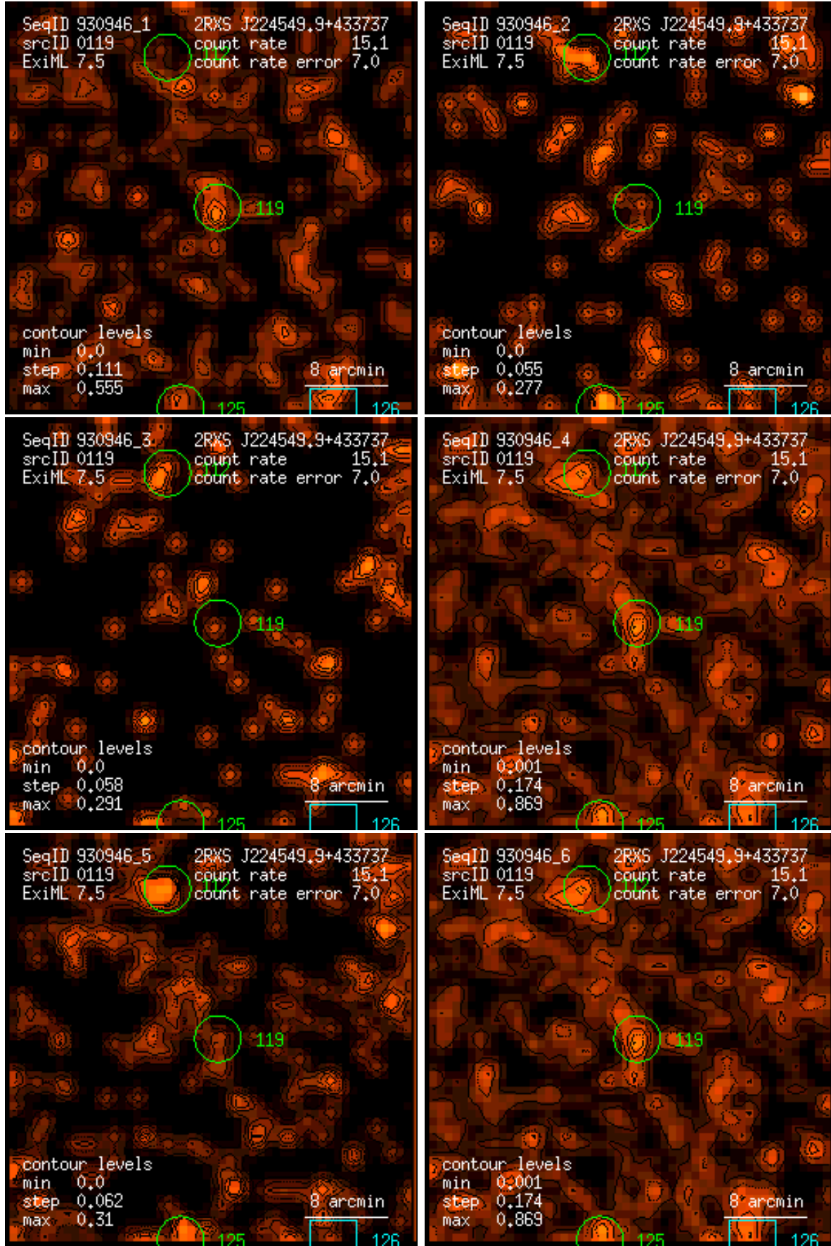
Figure 119: RASS 930946: detection 0119: band rate images, Gaussian filter: (1) PSPC channels 11 – 41, (2) 52 – 90, (3) 91 – 201, (4) 11 – 235, (5) 52 – 201, (6) 11 – 201. Broad band rates in counts/ks. Band rate contour levels in counts/ks/arcmin 2 .
