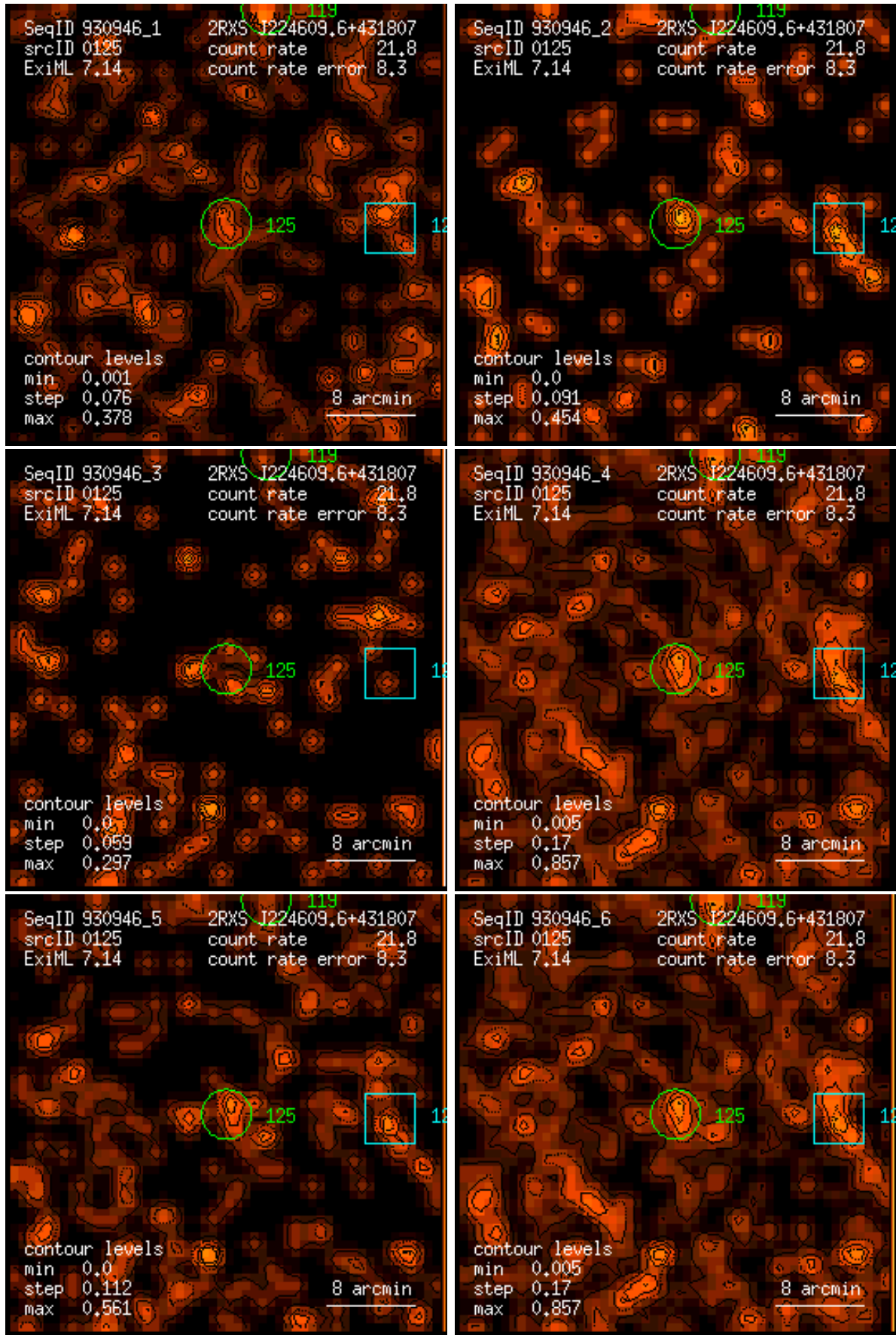
Figure 125: RASS 930946: detection 0125: band rate images, Gaussian filter: (1) PSPC channels 11 – 41, (2) 52 – 90, (3) 91 – 201, (4) 11 – 235, (5) 52 – 201, (6) 11 – 201. Broad band rates in counts/ks. Band rate contour levels in counts/ks/arcmin 2 .
