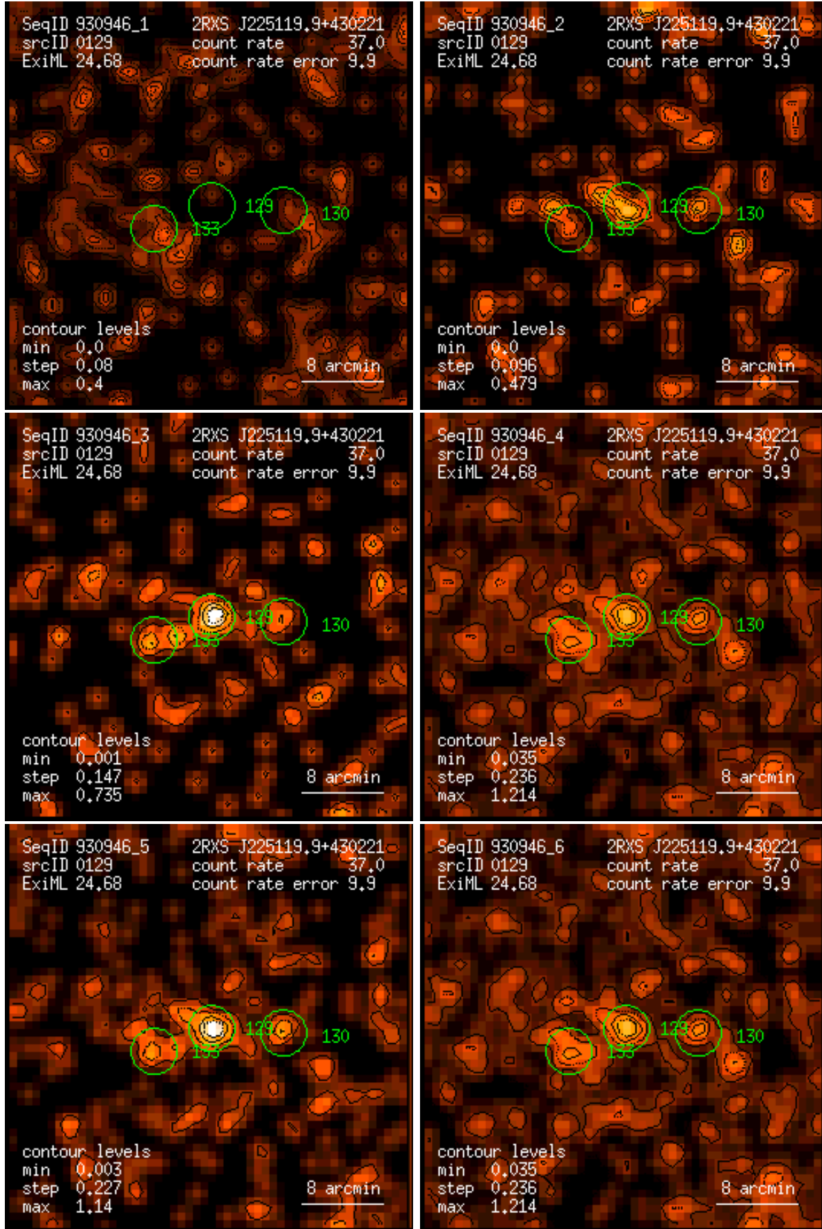
Figure 129: RASS 930946: detection 0129: band rate images, Gaussian filter: (1) PSPC channels 11 – 41, (2) 52 – 90, (3) 91 – 201, (4) 11 – 235, (5) 52 – 201, (6) 11 – 201. Broad band rates in counts/ks. Band rate contour levels in counts/ks/arcmin 2 .
