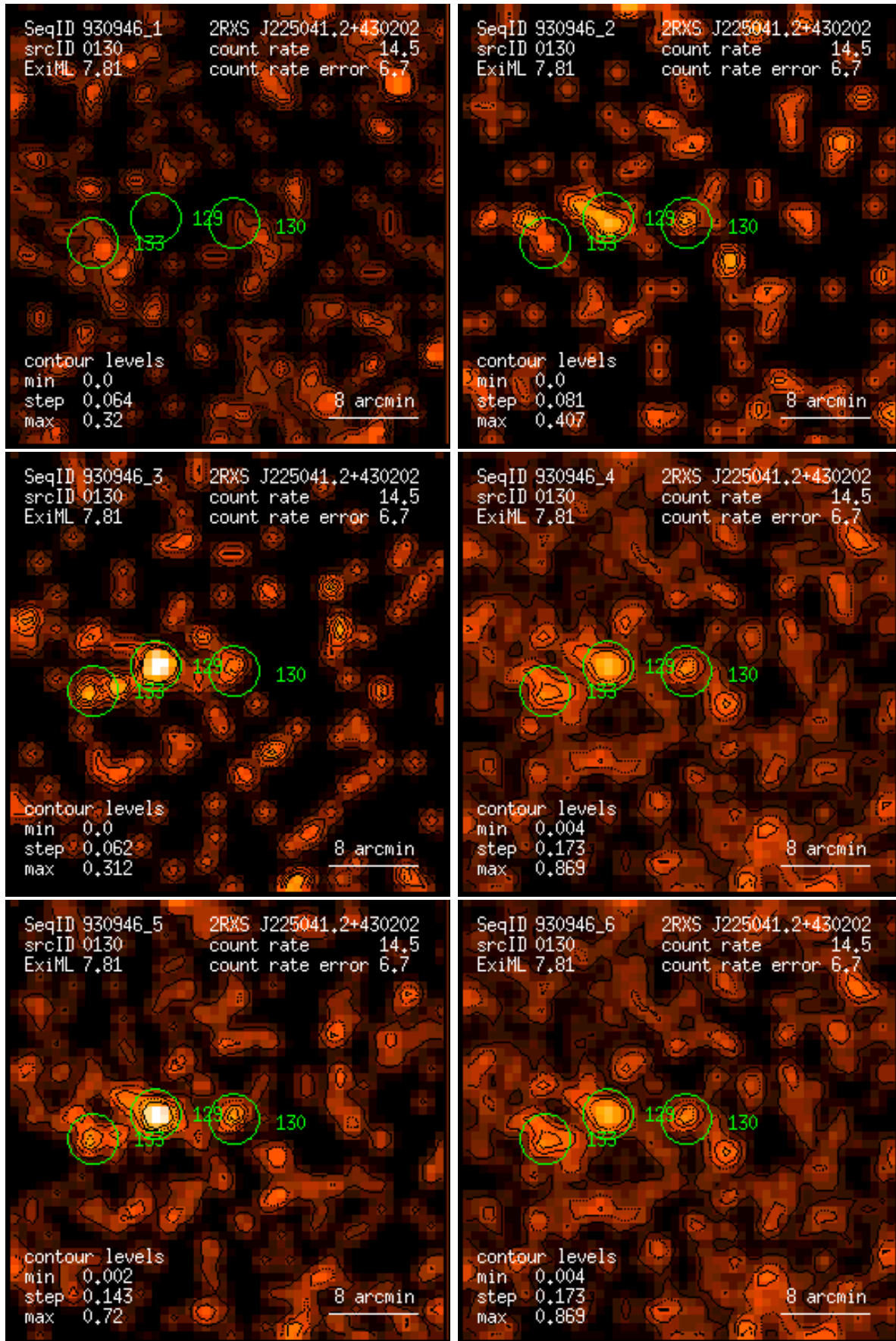
Figure 130: RASS 930946: detection 0130: band rate images, Gaussian filter: (1) PSPC channels 11 – 41, (2) 52 – 90, (3) 91 – 201, (4) 11 – 235, (5) 52 – 201, (6) 11 – 201. Broad band rates in counts/ks. Band rate contour levels in counts/ks/arcmin 2 .
