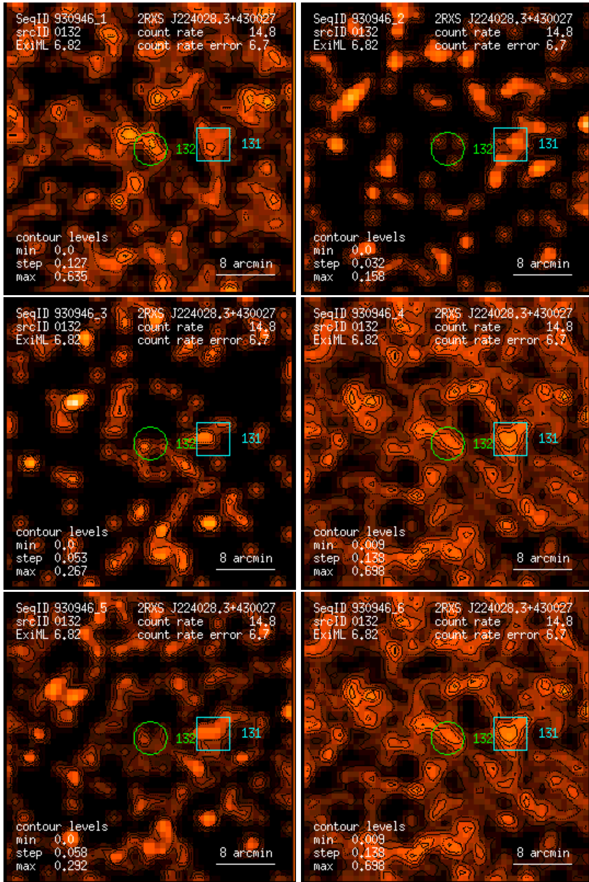
Figure 132: RASS 930946: detection 0132: band rate images, Gaussian filter: (1) PSPC channels 11 – 41, (2) 52 – 90, (3) 91 – 201, (4) 11 – 235, (5) 52 – 201, (6) 11 – 201. Broad band rates in counts/ks. Band rate contour levels in counts/ks/arcmin 2 .
