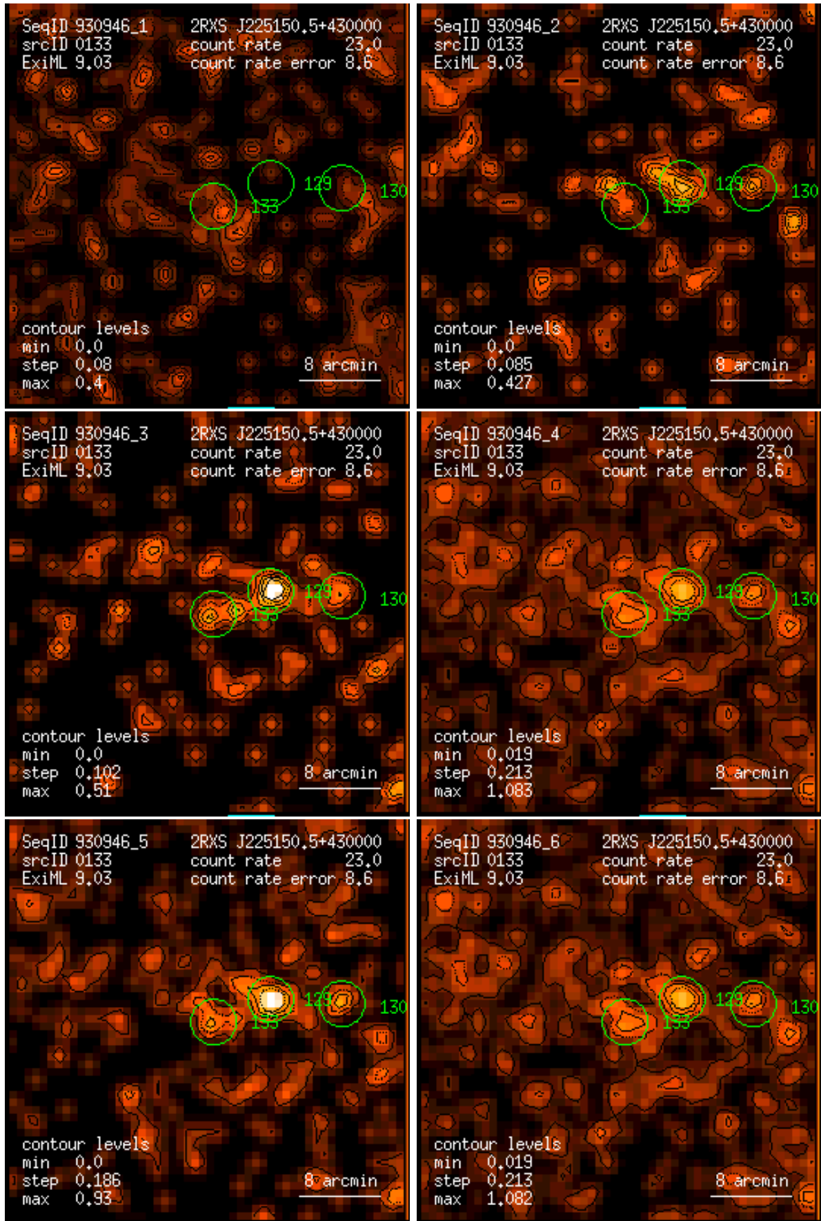
Figure 133: RASS 930946: detection 0133: band rate images, Gaussian filter: (1) PSPC channels 11 – 41, (2) 52 – 90, (3) 91 – 201, (4) 11 – 235, (5) 52 – 201, (6) 11 – 201. Broad band rates in counts/ks. Band rate contour levels in counts/ks/arcmin 2 .
