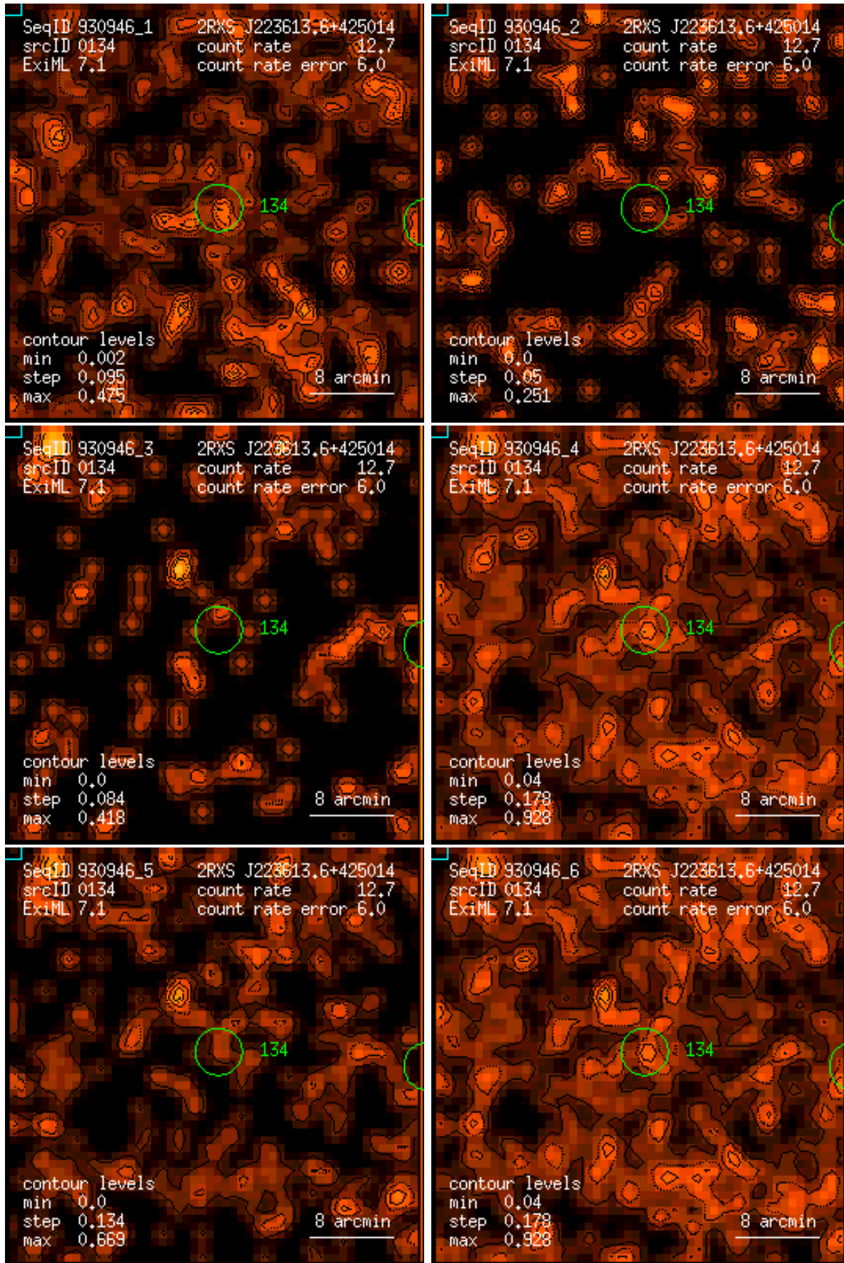
Figure 134: RASS 930946: detection 0134: band rate images, Gaussian filter: (1) PSPC channels 11 – 41, (2) 52 – 90, (3) 91 – 201, (4) 11 – 235, (5) 52 – 201, (6) 11 – 201. Broad band rates in counts/ks. Band rate contour levels in counts/ks/arcmin 2 .
