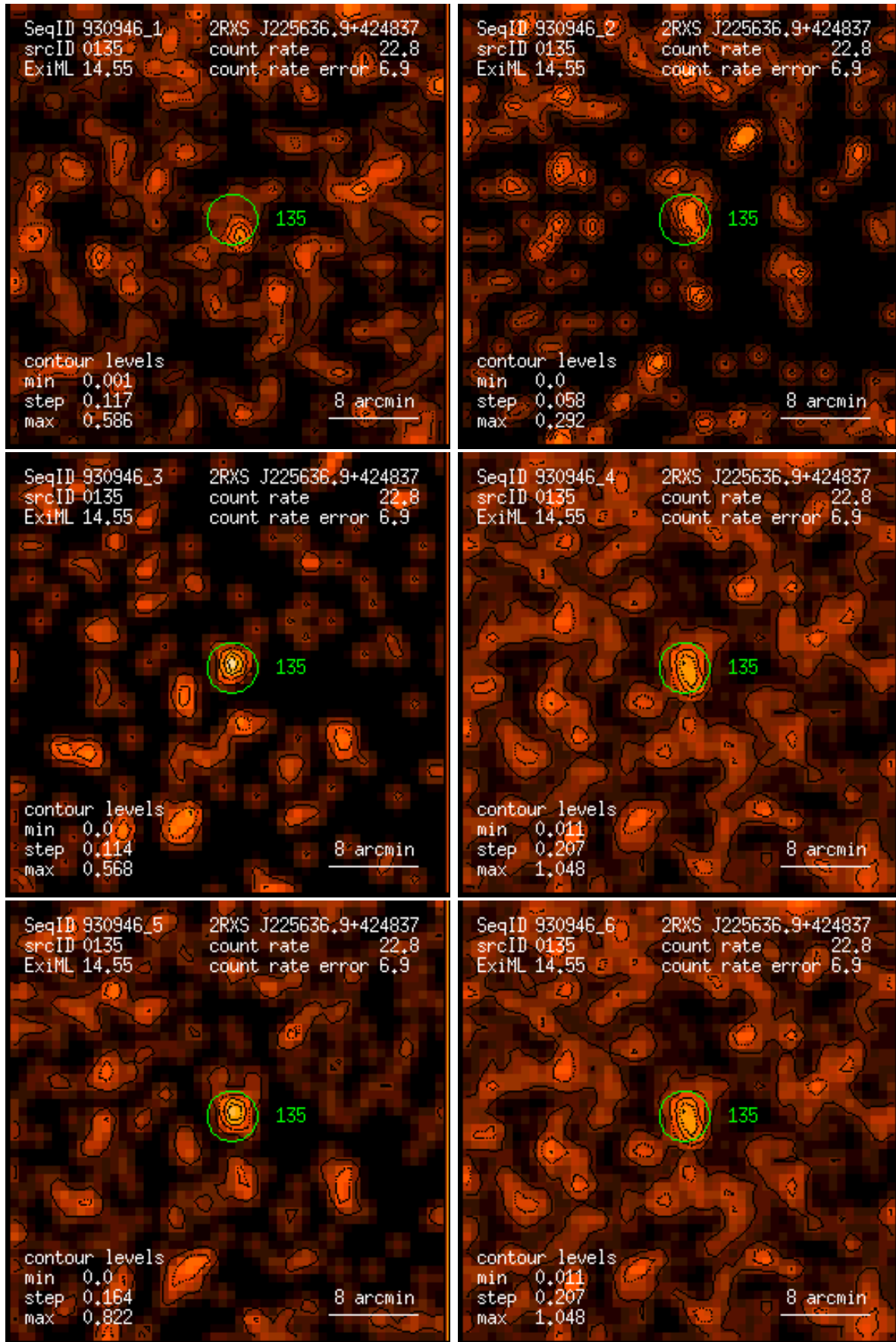
Figure 135: RASS 930946: detection 0135: band rate images, Gaussian filter: (1) PSPC channels 11 – 41, (2) 52 – 90, (3) 91 – 201, (4) 11 – 235, (5) 52 – 201, (6) 11 – 201. Broad band rates in counts/ks. Band rate contour levels in counts/ks/arcmin 2 .
