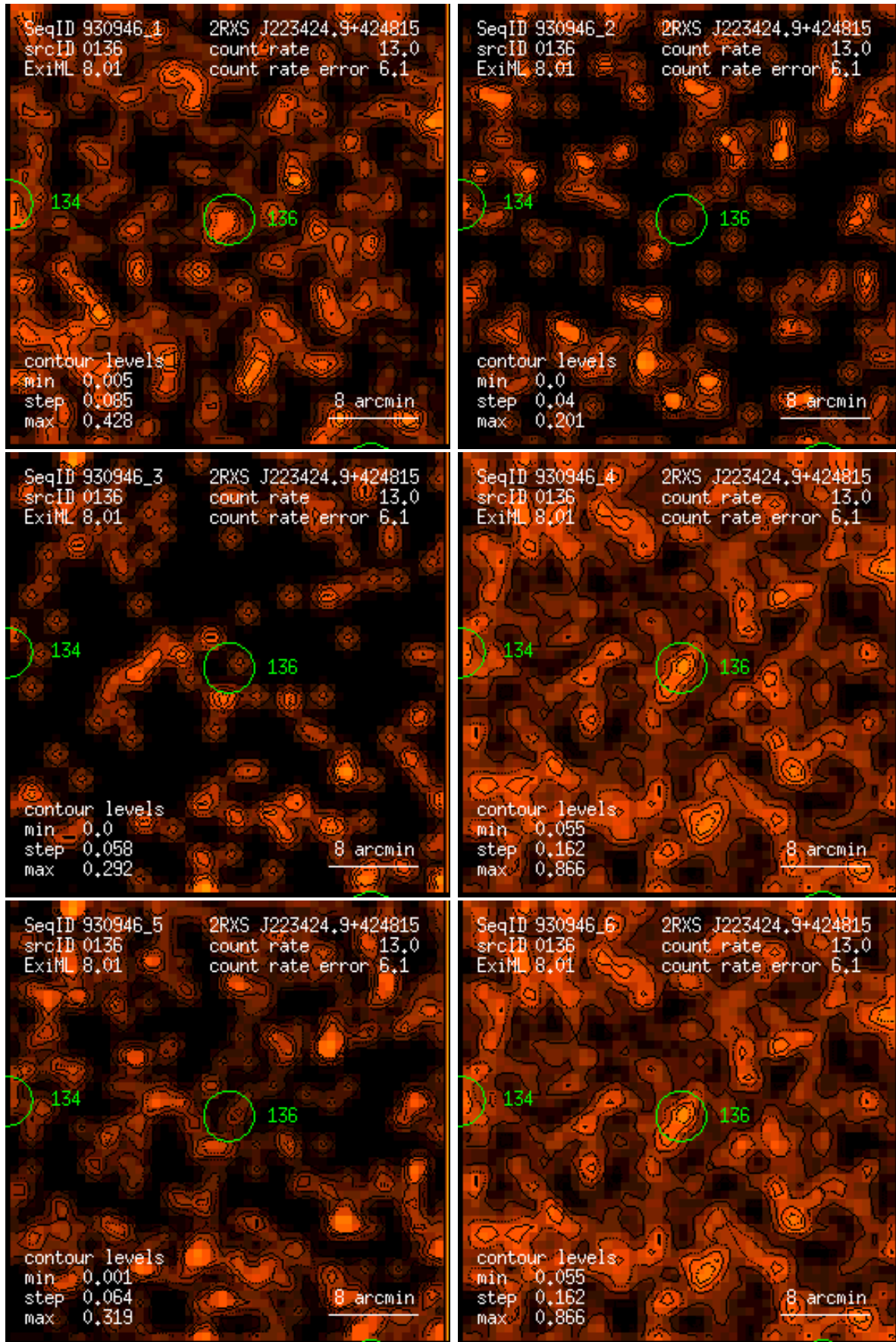
Figure 136: RASS 930946: detection 0136: band rate images, Gaussian filter: (1) PSPC channels 11 – 41, (2) 52 – 90, (3) 91 – 201, (4) 11 – 235, (5) 52 – 201, (6) 11 – 201. Broad band rates in counts/ks. Band rate contour levels in counts/ks/arcmin 2 .
