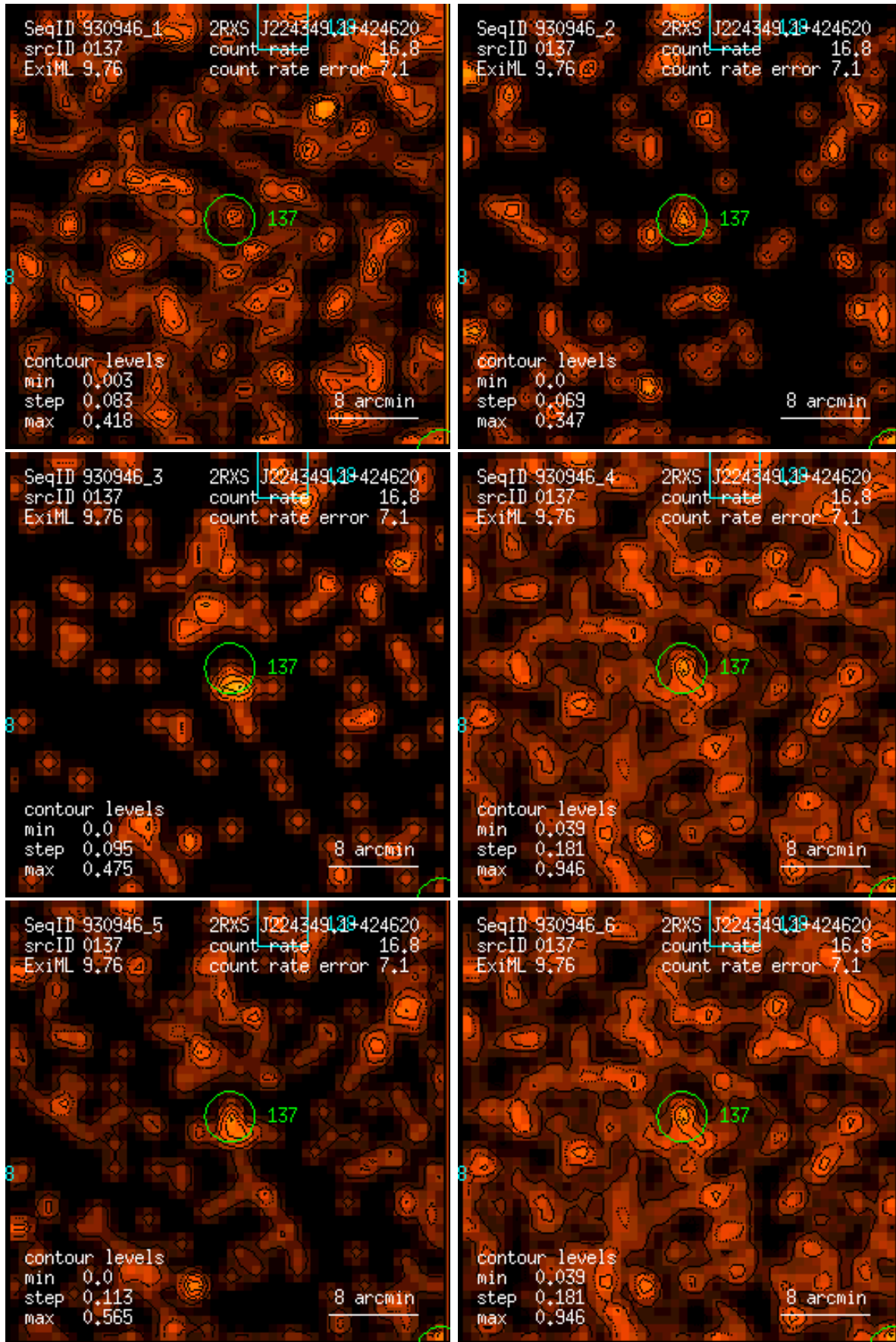
Figure 137: RASS 930946: detection 0137: band rate images, Gaussian filter: (1) PSPC channels 11 – 41, (2) 52 – 90, (3) 91 – 201, (4) 11 – 235, (5) 52 – 201, (6) 11 – 201. Broad band rates in counts/ks. Band rate contour levels in counts/ks/arcmin 2 .
