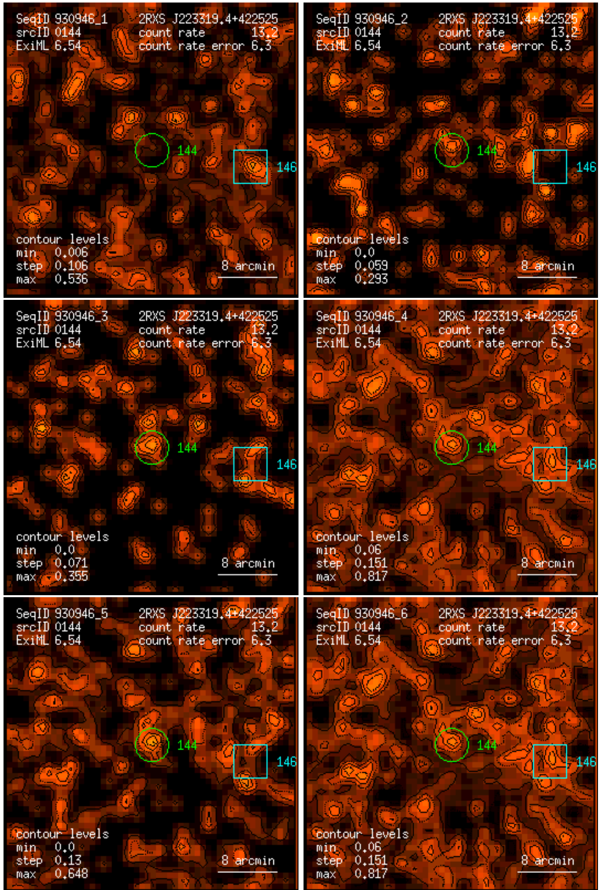
Figure 144: RASS 930946: detection 0144: band rate images, Gaussian filter: (1) PSPC channels 11 – 41, (2) 52 – 90, (3) 91 – 201, (4) 11 – 235, (5) 52 – 201, (6) 11 – 201. Broad band rates in counts/ks. Band rate contour levels in counts/ks/arcmin 2 .
