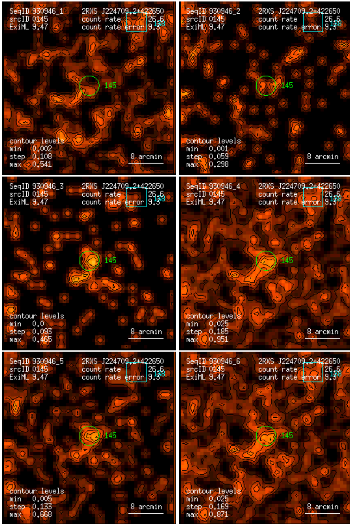
Figure 145: RASS 930946: detection 0145: band rate images, Gaussian filter: (1) PSPC channels 11 – 41, (2) 52 – 90, (3) 91 – 201, (4) 11 – 235, (5) 52 – 201, (6) 11 – 201. Broad band rates in counts/ks. Band rate contour levels in counts/ks/arcmin 2 .
