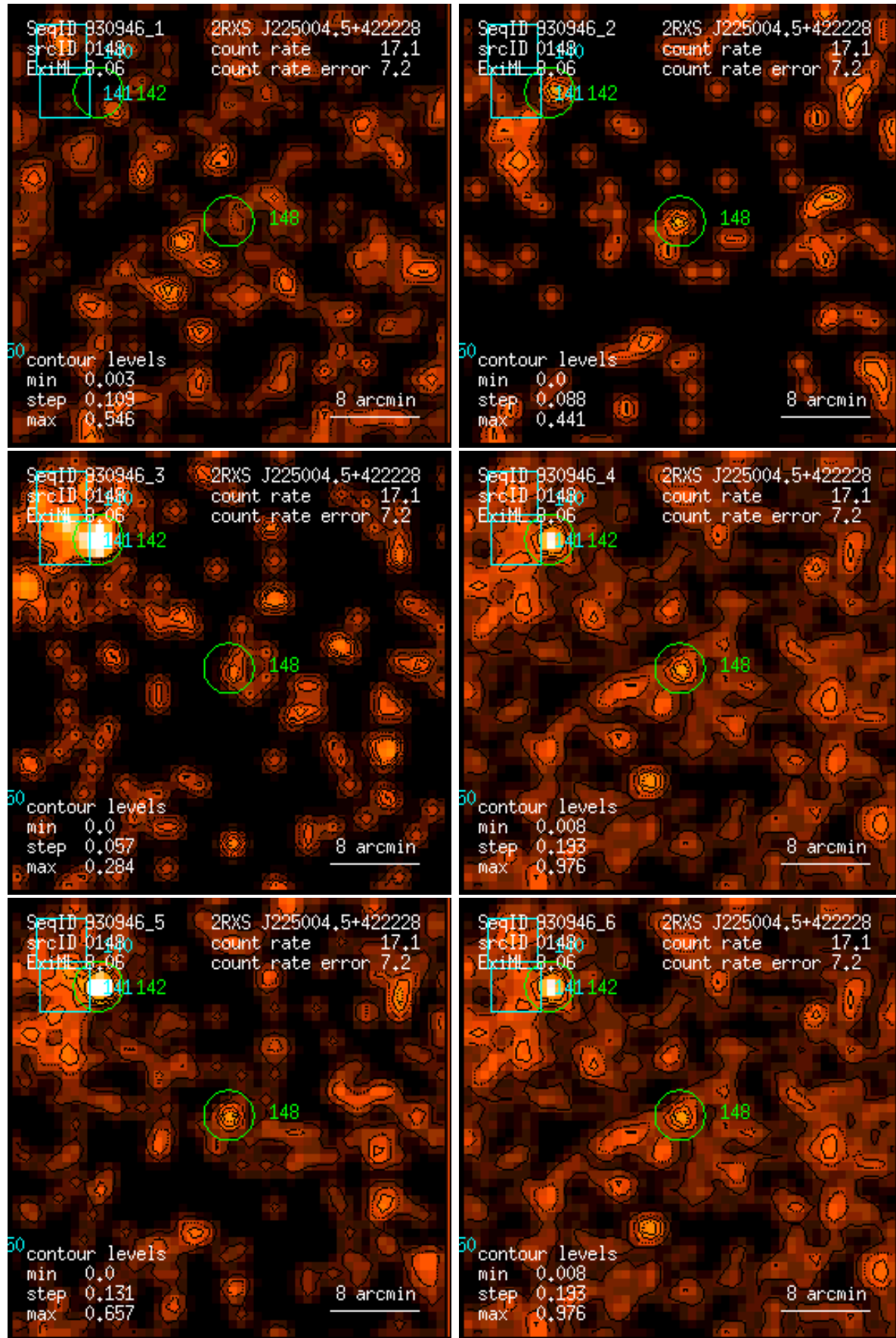
Figure 148: RASS 930946: detection 0148: band rate images, Gaussian filter: (1) PSPC channels 11 – 41, (2) 52 – 90, (3) 91 – 201, (4) 11 – 235, (5) 52 – 201, (6) 11 – 201. Broad band rates in counts/ks. Band rate contour levels in counts/ks/arcmin 2 .
