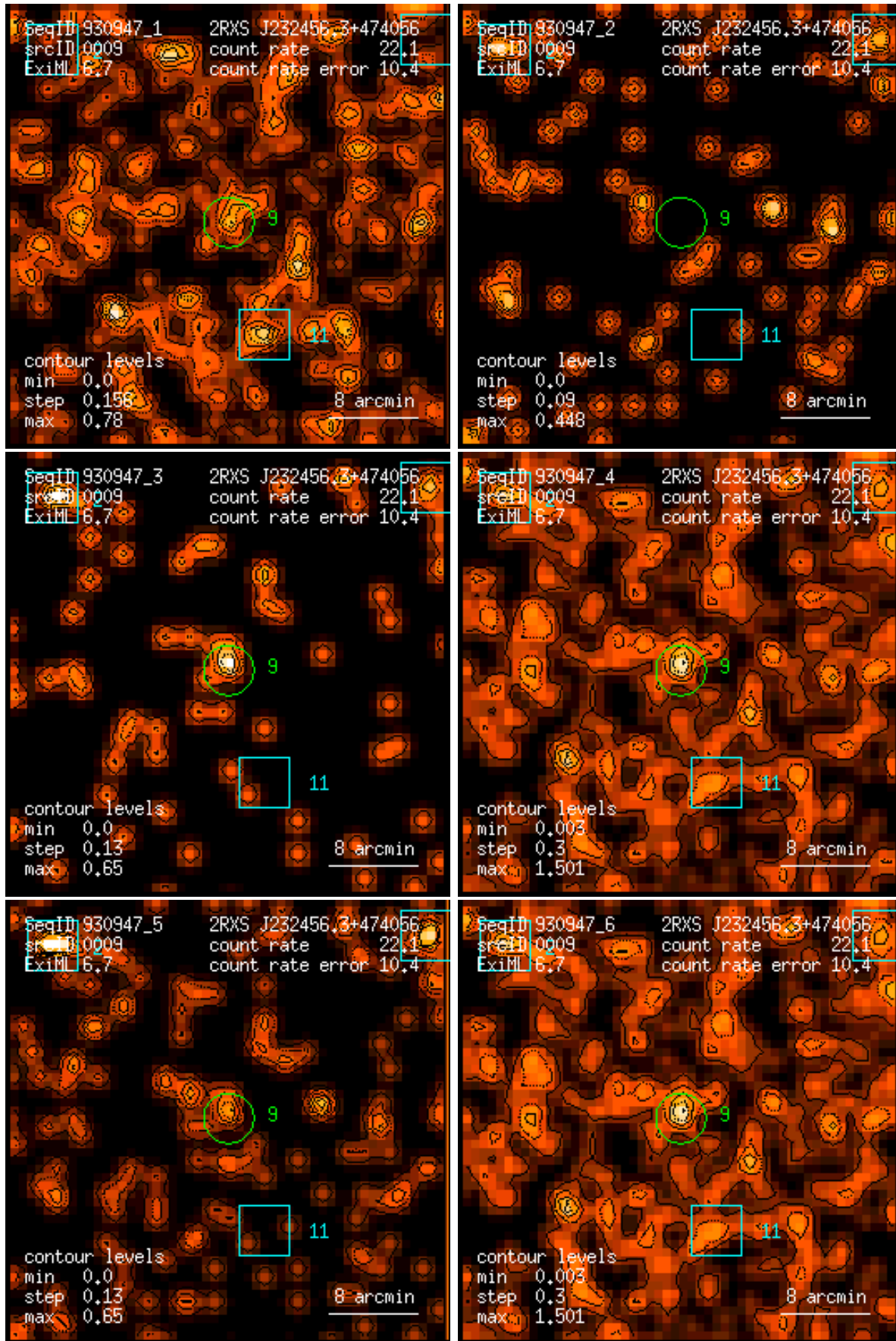
Figure 9: RASS 930947: detection 0009: band rate images, Gaussian filter: (1) PSPC channels 11 – 41, (2) 52 – 90, (3) 91 – 201, (4) 11 – 235, (5) 52 – 201, (6) 11 – 201. Broad band rates in counts/ks. Band rate contour levels in counts/ks/arcmin 2 .
