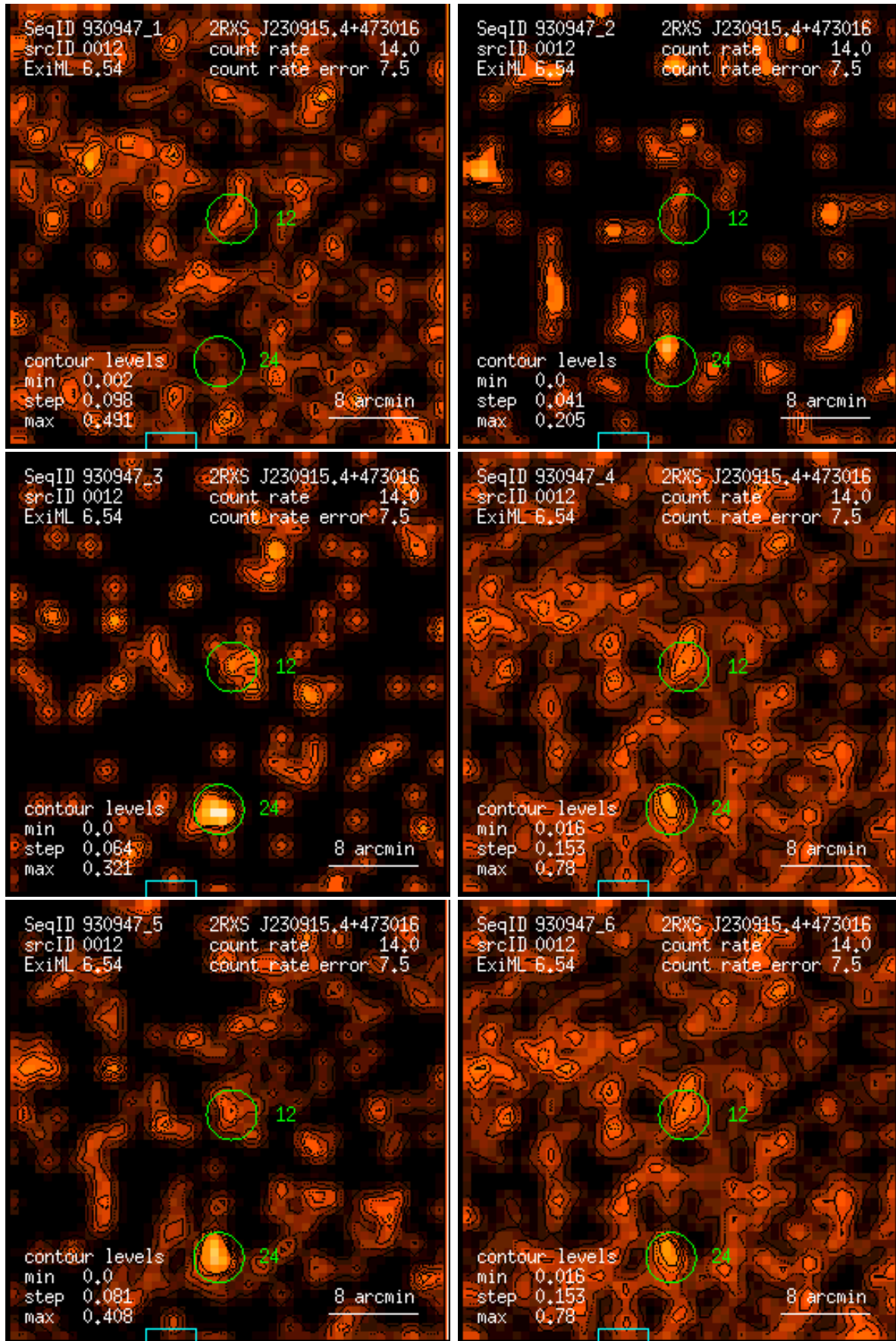
Figure 12: RASS 930947: detection 0012: band rate images, Gaussian filter: (1) PSPC channels 11 – 41, (2) 52 – 90, (3) 91 – 201, (4) 11 – 235, (5) 52 – 201, (6) 11 – 201. Broad band rates in counts/ks. Band rate contour levels in counts/ks/arcmin 2 .
