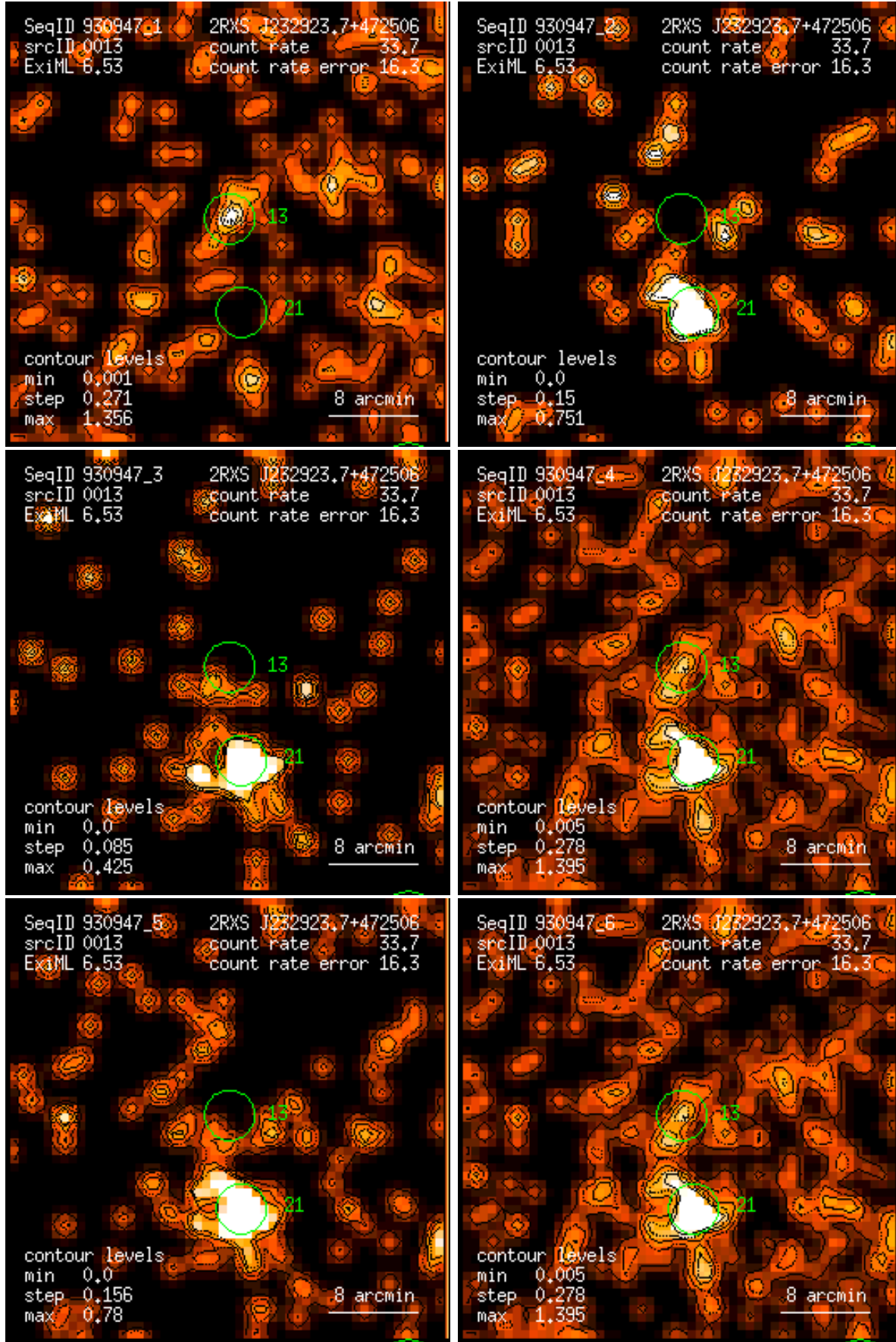
Figure 13: RASS 930947: detection 0013: band rate images, Gaussian filter: (1) PSPC channels 11 – 41, (2) 52 – 90, (3) 91 – 201, (4) 11 – 235, (5) 52 – 201, (6) 11 – 201. Broad band rates in counts/ks. Band rate contour levels in counts/ks/arcmin 2 .
