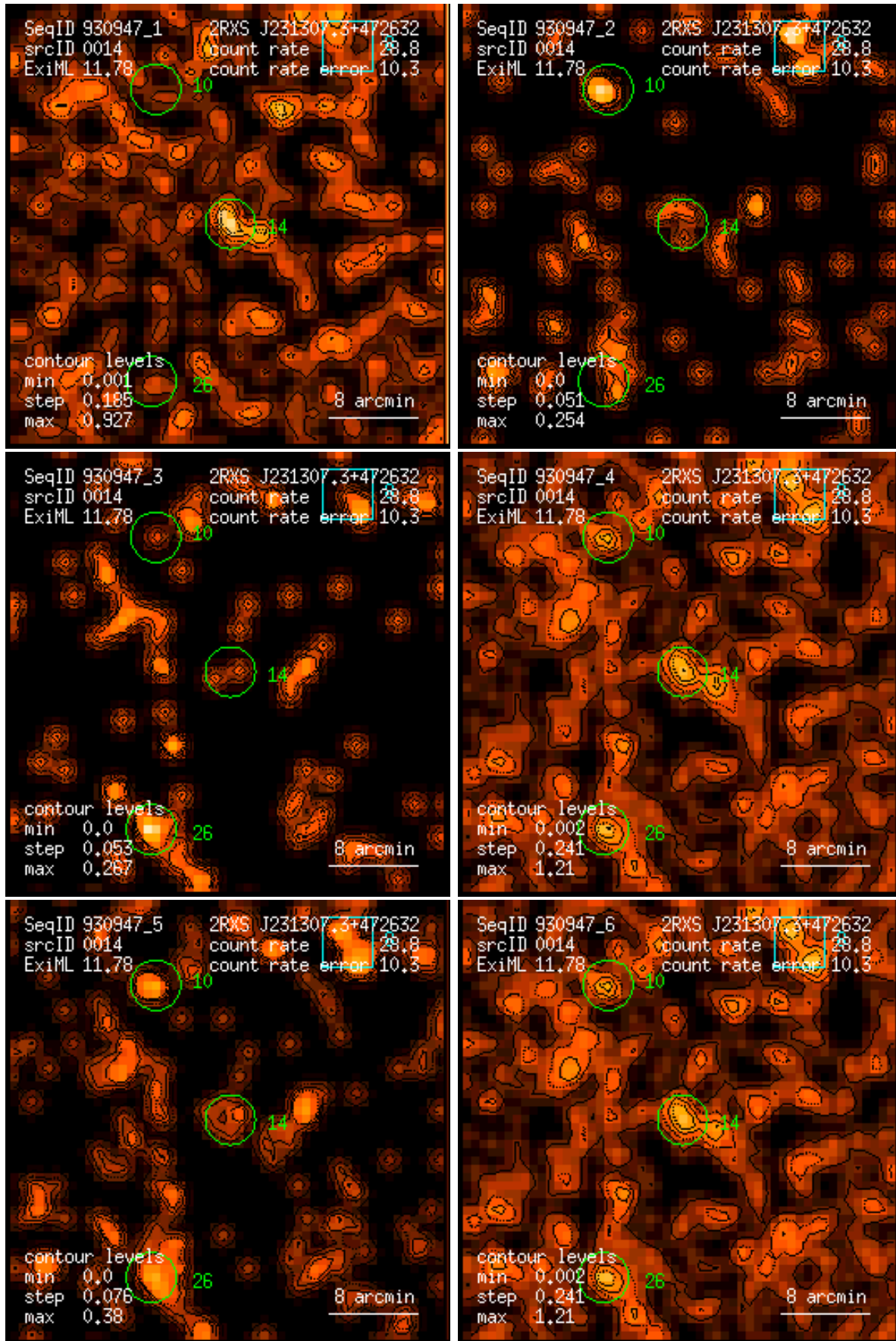
Figure 14: RASS 930947: detection 0014: band rate images, Gaussian filter: (1) PSPC channels 11 – 41, (2) 52 – 90, (3) 91 – 201, (4) 11 – 235, (5) 52 – 201, (6) 11 – 201. Broad band rates in counts/ks. Band rate contour levels in counts/ks/arcmin 2 .
