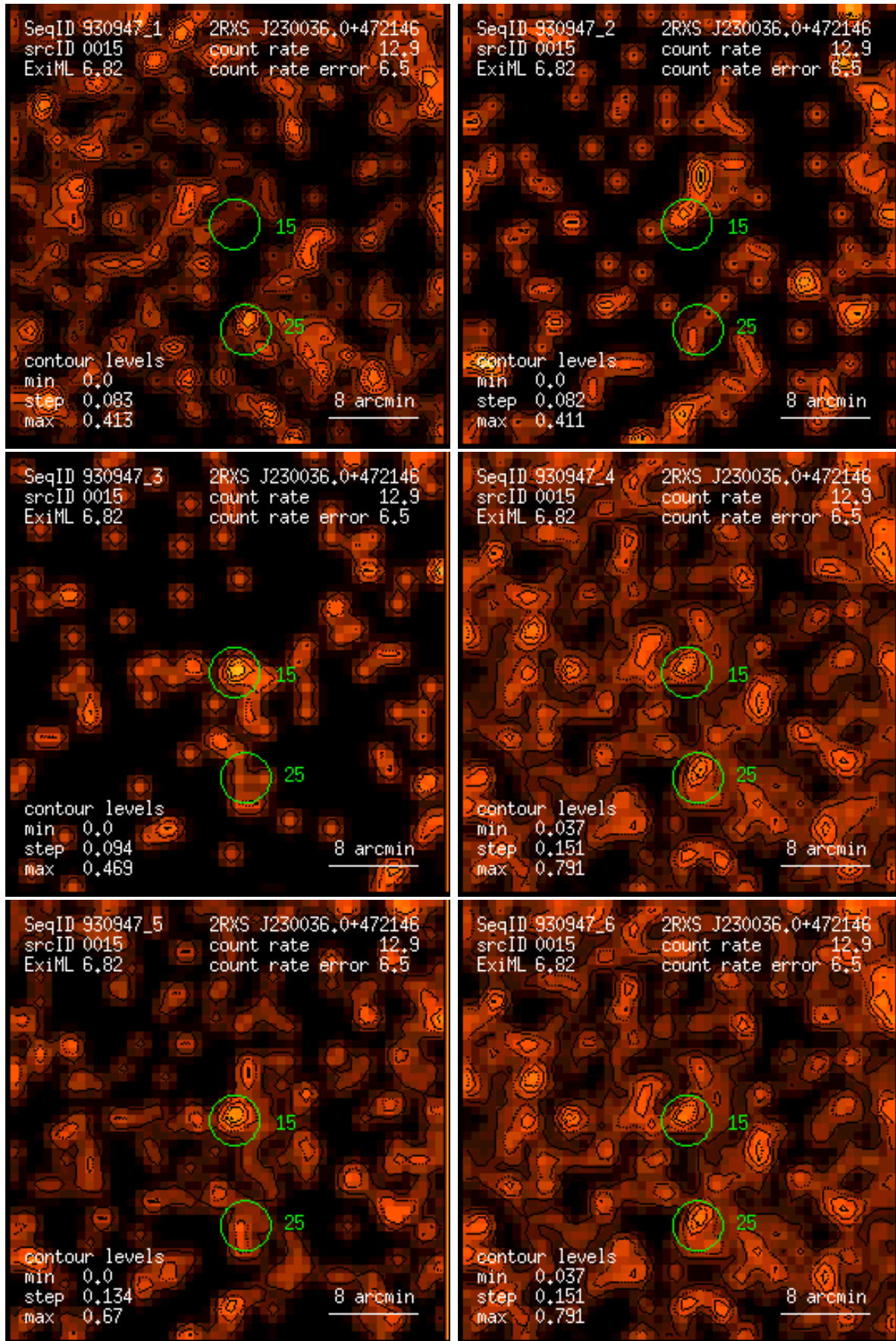
Figure 15: RASS 930947: detection 0015: band rate images, Gaussian filter: (1) PSPC channels 11 – 41, (2) 52 – 90, (3) 91 – 201, (4) 11 – 235, (5) 52 – 201, (6) 11 – 201. Broad band rates in counts/ks. Band rate contour levels in counts/ks/arcmin 2 .
