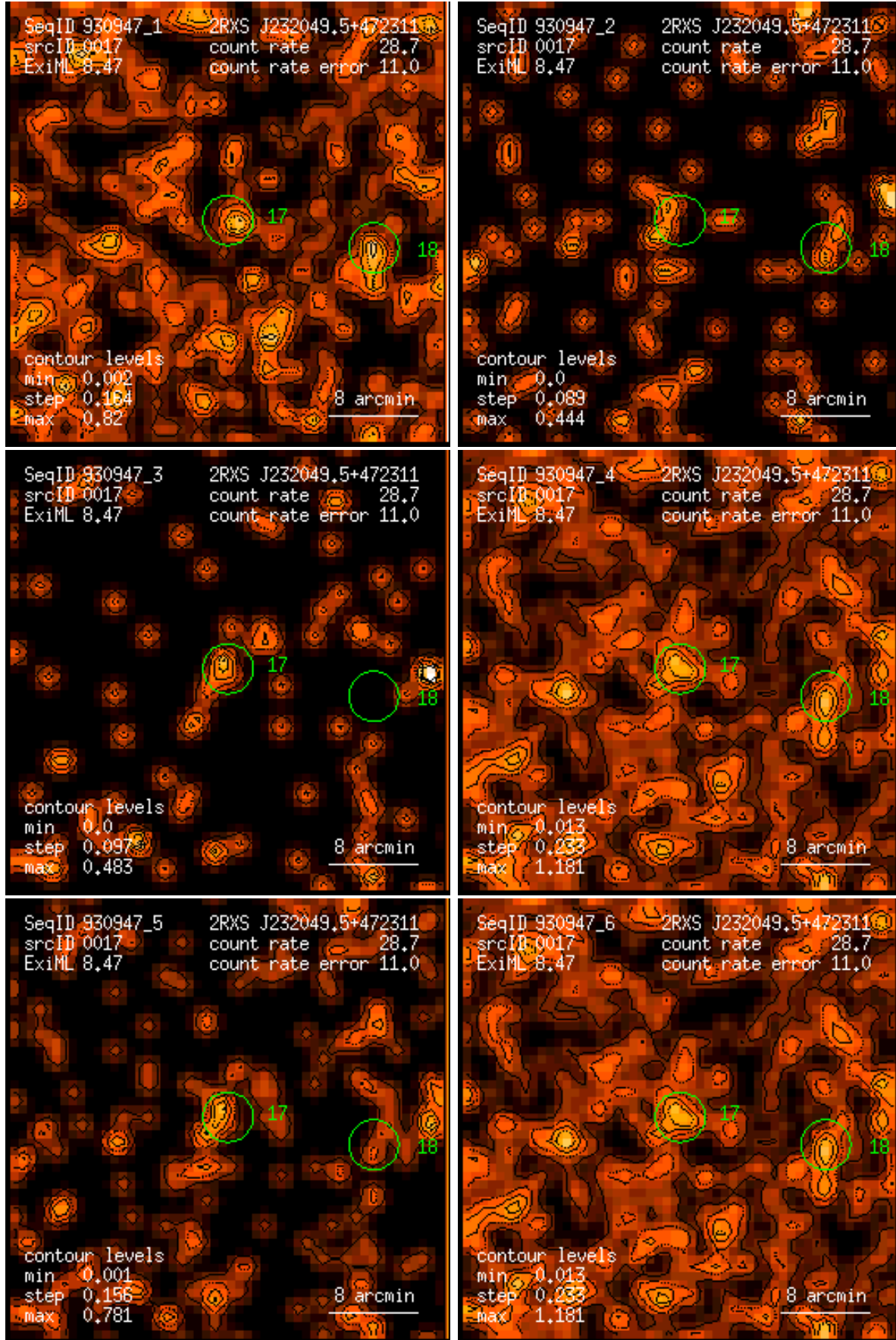
Figure 17: RASS 930947: detection 0017: band rate images, Gaussian filter: (1) PSPC channels 11 – 41, (2) 52 – 90, (3) 91 – 201, (4) 11 – 235, (5) 52 – 201, (6) 11 – 201. Broad band rates in counts/ks. Band rate contour levels in counts/ks/arcmin 2 .
