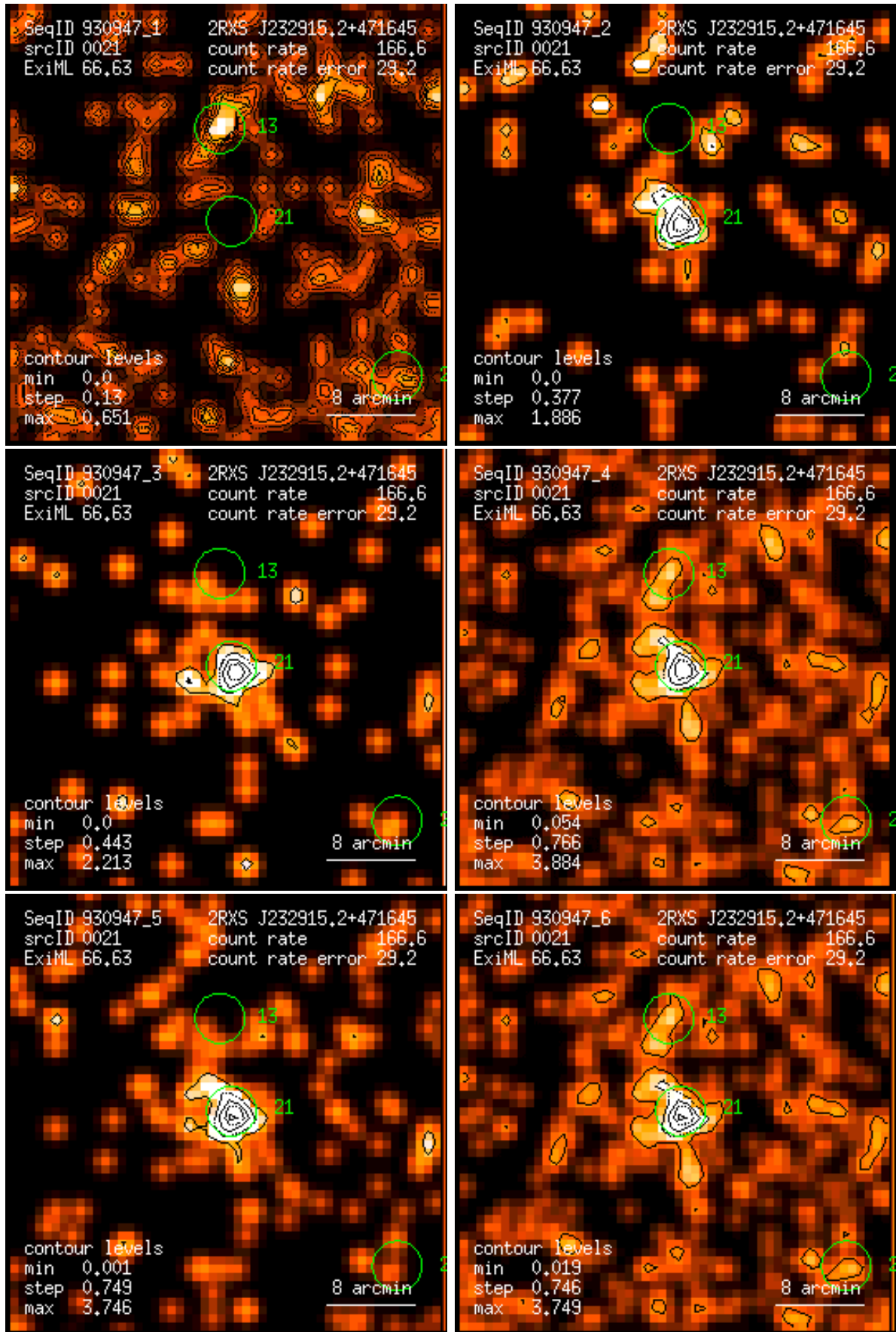
Figure 21: RASS 930947: detection 0021: band rate images, Gaussian filter: (1) PSPC channels 11 – 41, (2) 52 – 90, (3) 91 – 201, (4) 11 – 235, (5) 52 – 201, (6) 11 – 201. Broad band rates in counts/ks. Band rate contour levels in counts/ks/arcmin 2 .
